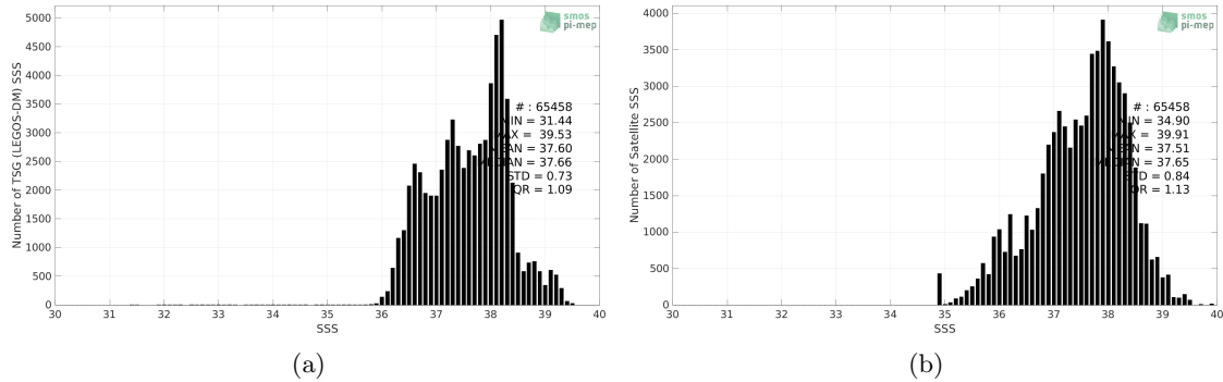
Figure 2: Histograms of SSS from TSG (LEGOS-DM) (a) and SMAP SSS L3 v5 - Monthly (RSS) (b) considering all match-up pairs per bins of 0.1 over the Mediterranean Sea Pi-MEP region and for the full satellite product period.
