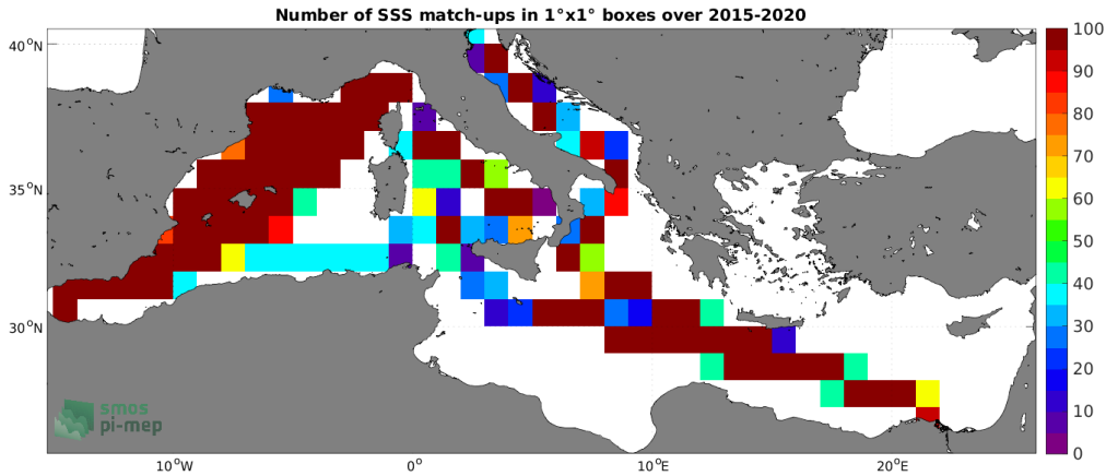
Figure 4: Number of SSS match-ups between TSG (LEGOS-DM) SSS and the SMAP SSS L3 v5 - Monthly (RSS) SSS product for the Mediterranean Sea Pi-MEP region over 1^\circ \times 1^\circ boxes and for the full satellite product period.
