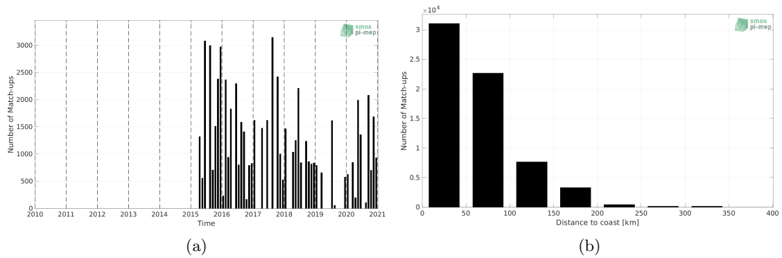
Figure 1: Number of match-ups between TSG (LEGOS-DM) and SMAP SSS L3 v5 - Monthly (RSS) SSS as a function of time (a) and as function of the distance to coast (b) over the Mediterranean Sea Pi-MEP region and for the full satellite product period.
