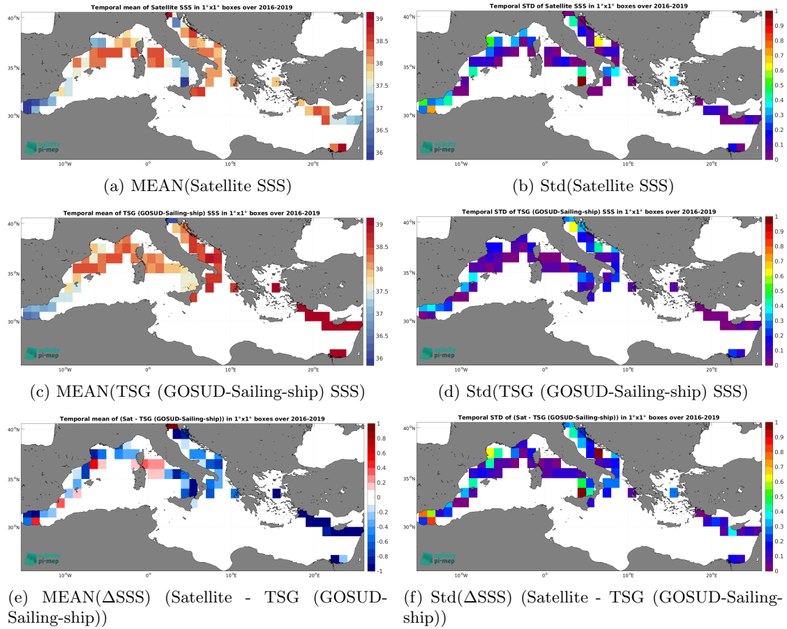
Figure 6: Temporal mean (left) and Std (right) of SSS from SMAP SSS L3 v5 - Monthly (RSS) (top), TSG (GOSUD-Sailing-ship) (middle), and of \Delta SSS (Satellite - TSG (GOSUD-Sailing-ship)). Only match-up pairs are used to generate these maps.
