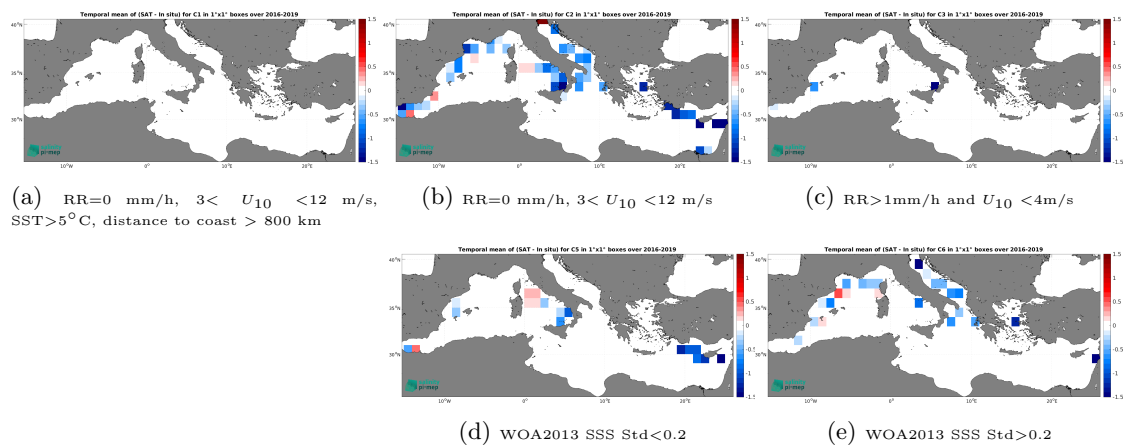
Figure 12: Temporal mean gridded over spatial boxes of size 1^\circ \times 1^\circ of \Delta SSS (SMAP SSS L3 v5 - Monthly (RSS) - TSG (GOSUD-Sailing-ship)) for 5 different subdatasets corresponding to:RR=0 mm/h, 3 < U_{10} < 12 m/s, SST >5^\circ\text{C} , distance to coast > 800 km (a), RR=0 mm/h, 3 < U_{10} < 12 m/s (b), RR >1 mm/h and U_{10} < 4 m/s (c), WOA2013 SSS Std <0.2 (d), WOA2013 SSS Std >0.2 (e).
