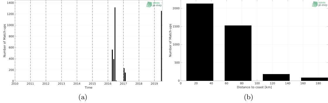
Figure 1: Number of match-ups between TSG (GOSUD-Sailing-ship) and SMAP SSS L3 v5 - Monthly (RSS) SSS as a function of time (a) and as function of the distance to coast (b) over the Mediterranean Sea Pi-MEP region and for the full satellite product period.
