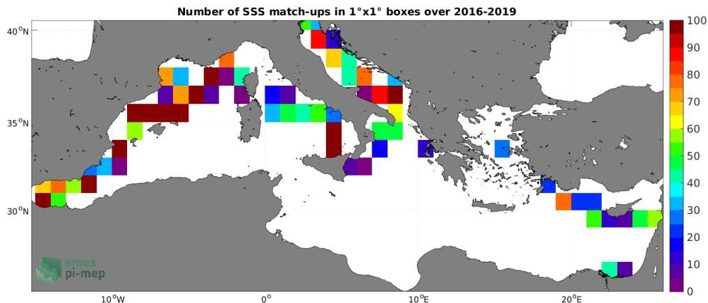
Figure 4: Number of SSS match-ups between TSG (GOSUD-Sailing-ship) SSS and the SMAP SSS L3 v5 - Monthly (RSS) SSS product for the Mediterranean Sea Pi-MEP region over 1^\circ \times 1^\circ boxes and for the full satellite product period.
