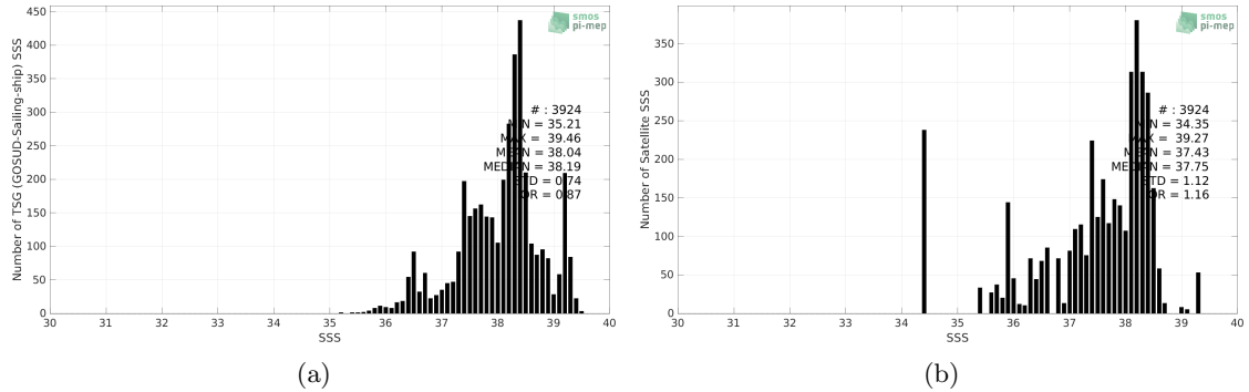
Figure 2: Histograms of SSS from TSG (GOSUD-Sailing-ship) (a) and SMAP SSS L3 v5 - Monthly (RSS) (b) considering all match-up pairs per bins of 0.1 over the Mediterranean Sea Pi-MEP region and for the full satellite product period.
