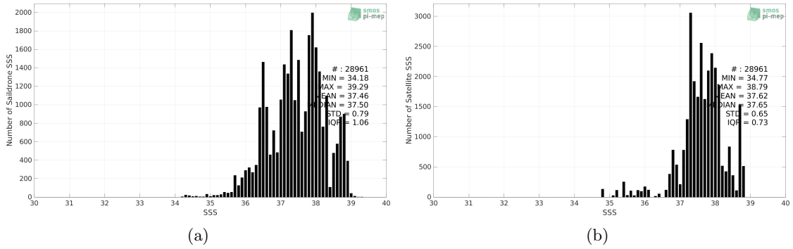
Figure 2: Histograms of SSS from Saildrone (a) and SMAP SSS L3 v5 - Monthly (RSS) (b) considering all match-up pairs per bins of 0.1 over the Mediterranean Sea Pi-MEP region and for the full satellite product period.
