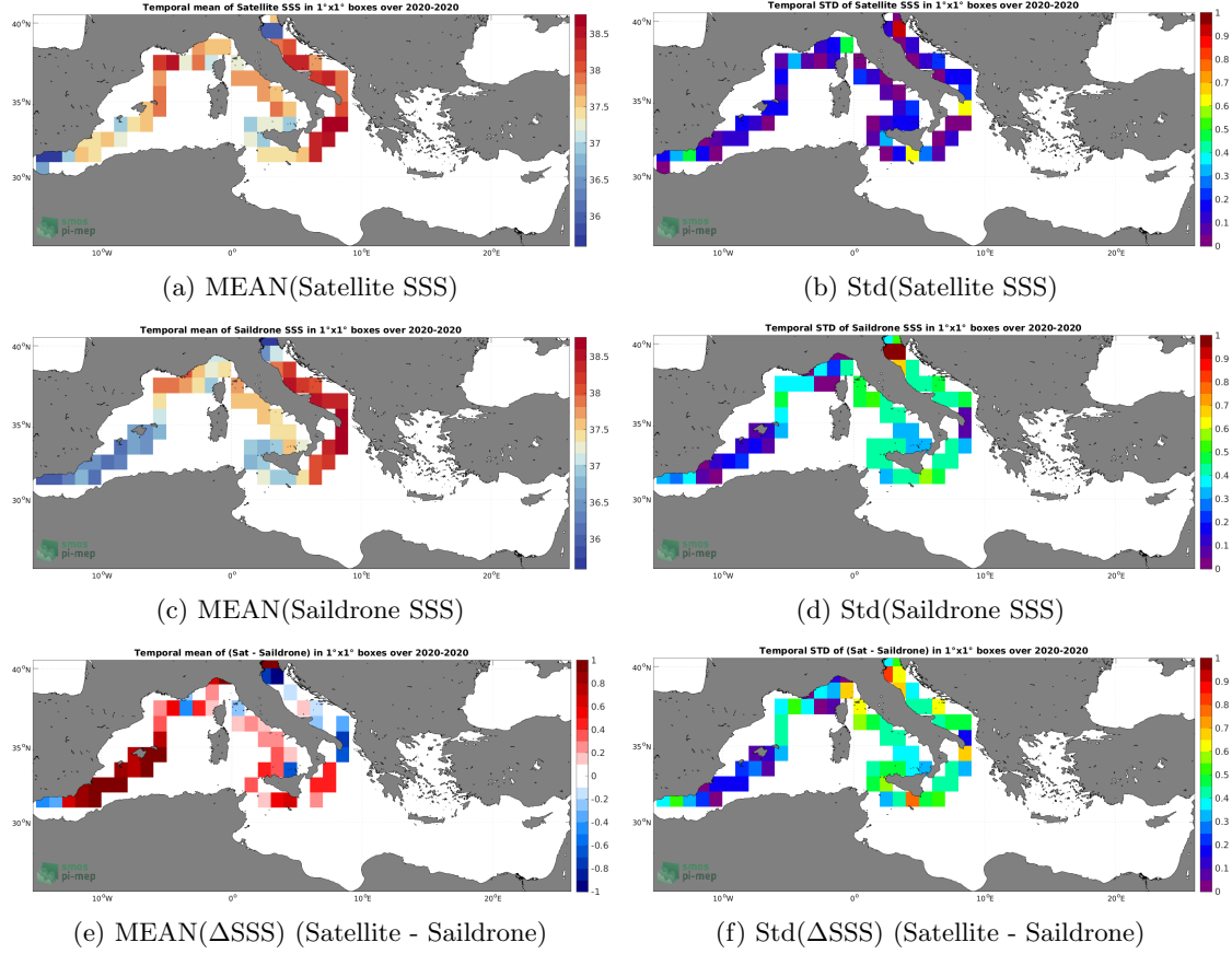
Figure 6: Temporal mean (left) and Std (right) of SSS from SMAP SSS L3 v5 - Monthly (RSS) (top), Saildrone (middle), and of \Delta\text{SSS} (Satellite - Saildrone). Only match-up pairs are used to generate these maps.
