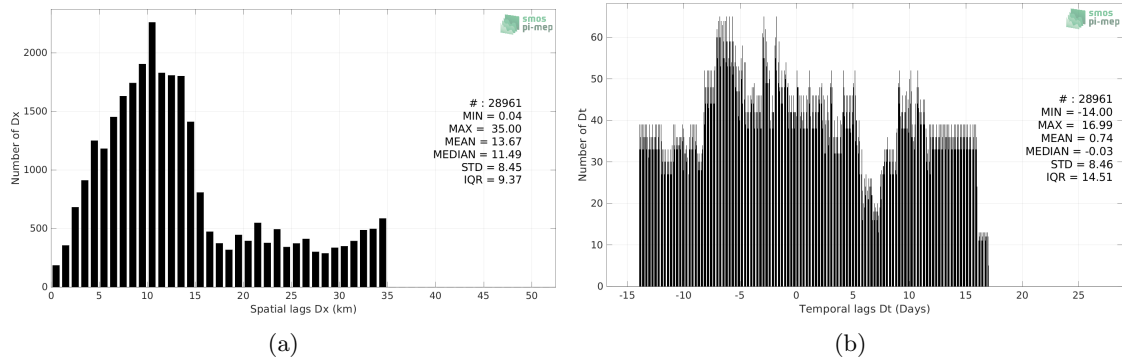
Figure 5: Histograms of the spatial (a) and temporal (b) lags between the location/time of the Sailsdrone measurement and the date of the corresponding SMAP SSS L3 v5 - Monthly (RSS) SSS pixel.
