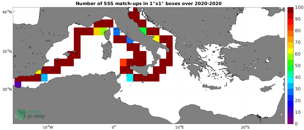
Figure 4: Number of SSS match-ups between Sailsdrone SSS and the SMAP SSS L3 v5 - Monthly (RSS) SSS product for the Mediterranean Sea Pi-MEP region over 1^\circ \times 1^\circ boxes and for the full satellite product period.
