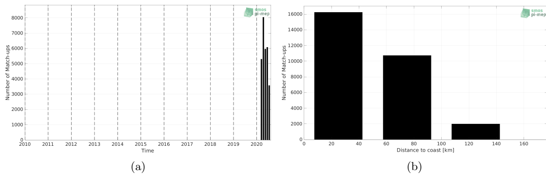
Figure 1: Number of match-ups between Sairdrone and SMAP SSS L3 v5 - Monthly (RSS) SSS as a function of time (a) and as function of the distance to coast (b) over the Mediterranean Sea Pi-MEP region and for the full satellite product period.
