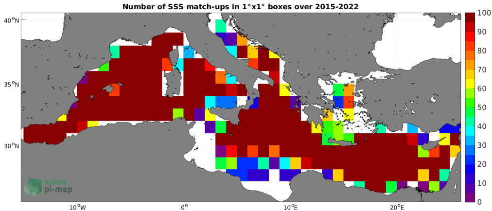
Figure 4: Number of SSS match-ups between Argo SSS and the SMAP SSS L3 v5 - Monthly (RSS) SSS product for the Mediterranean Sea Pi-MEP region over 1^{\circ} \times 1^{\circ} boxes and for the full satellite product period.
