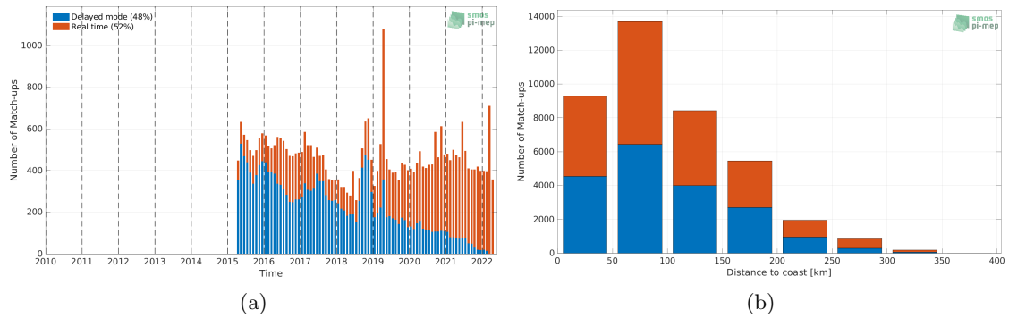
Figure 1: Number of match-ups between Argo and SMAP SSS L3 v5 - Monthly (RSS) SSS as a function of time (a) and as function of the distance to coast (b) over the Mediterranean Sea Pi-MEP region and for the full satellite product period.
