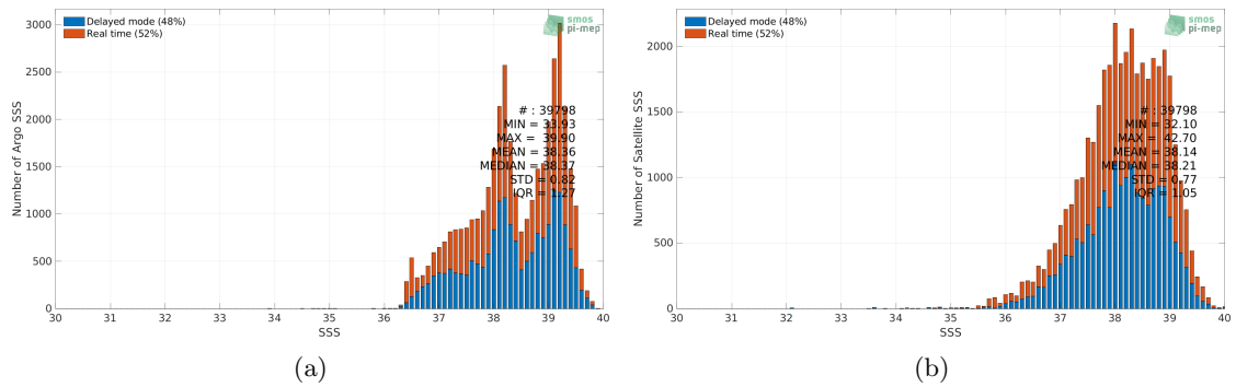
Figure 2: Histograms of SSS from Argo (a) and SMAP SSS L3 v5 - Monthly (RSS) (b) considering all match-up pairs per bins of 0.1 over the Mediterranean Sea Pi-MEP region and for the full satellite product period.
