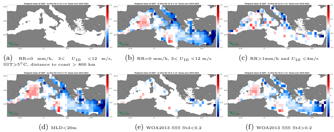
Figure 12: Temporal mean gridded over spatial boxes of size 1^\circ \times 1^\circ of \Delta SSS (SMAP SSS L3 v5 - Monthly (RSS) - Argo) for 6 different subdatasets corresponding to:RR=0 mm/h, 3 < U_{10} < 12 m/s, SST >5^\circ C, distance to coast > 800 km (a), RR=0 mm/h, 3 < U_{10} < 12 m/s (b), RR >1 mm/h and U_{10} < 4 m/s (c),MLD <20 m (d),WOA2013 SSS Std <0.2 (e),WOA2013 SSS Std >0.2 (f).
