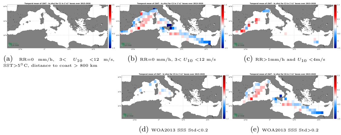
Figure 12: Temporal mean gridded over spatial boxes of size 1^\circ \times 1^\circ of \Delta\text{SSS} (SMAP SSS L3 v4 - 8-Day running (RSS) - TSG (LEGOS-DM)) for 5 different subdatasets corresponding to:RR=0 mm/h, 3 < U_{10} < 12 m/s, SST >5^\circ\text{C} , distance to coast > 800 km (a), RR=0 mm/h, 3 < U_{10} < 12 m/s (b), RR >1 mm/h and U_{10} < 4 m/s (c), WOA2013 SSS Std <0.2 (d), WOA2013 SSS Std >0.2 (e).
