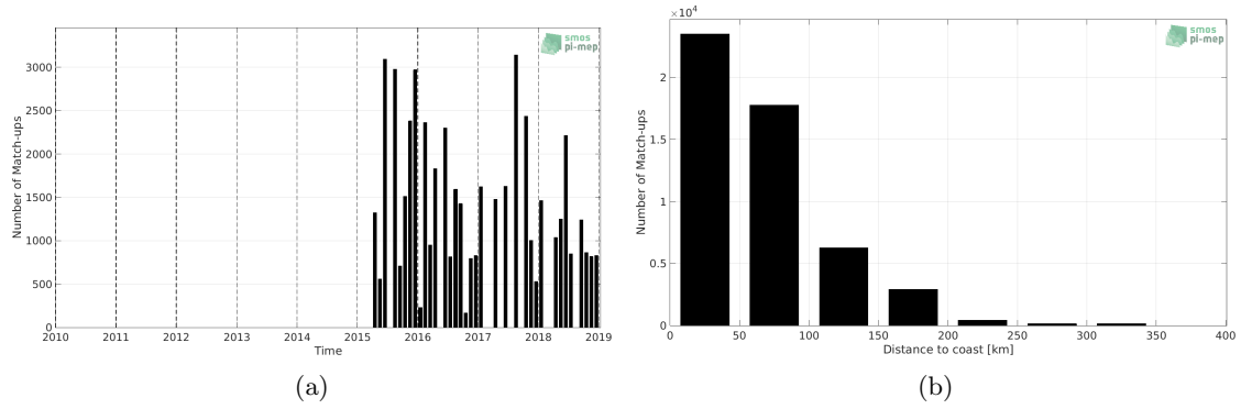
Figure 1: Number of match-ups between TSG (LEGOS-DM) and SMAP SSS L3 v4 - 8-Day running (RSS) SSS as a function of time (a) and as function of the distance to coast (b) over the Mediterranean Sea Pi-MEP region and for the full satellite product period.
