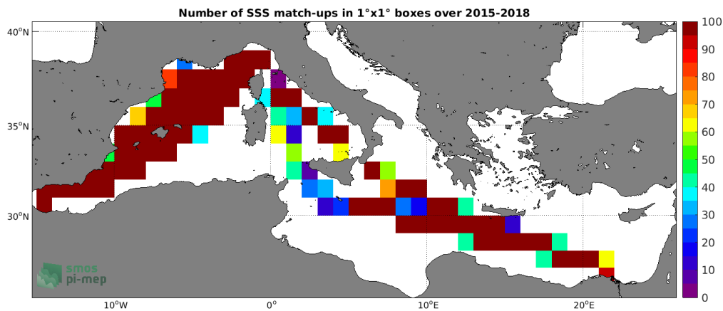
Figure 4: Number of SSS match-ups between TSG (LEGOS-DM) SSS and the SMAP SSS L3 v4 - 8-Day running (RSS) SSS product for the Mediterranean Sea Pi-MEP region over 1^\circ \times 1^\circ boxes and for the full satellite product period.
