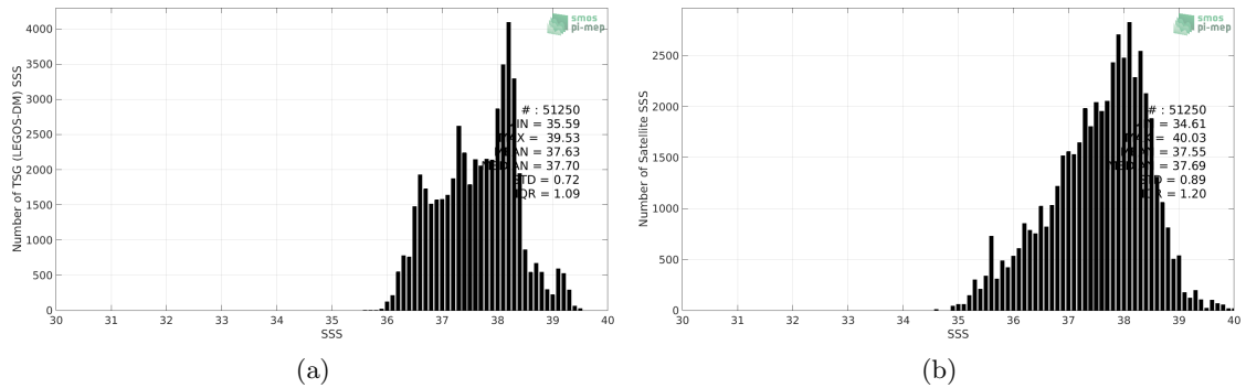
Figure 2: Histograms of SSS from TSG (LEGOS-DM) (a) and SMAP SSS L3 v4 - 8-Day running (RSS) (b) considering all match-up pairs per bins of 0.1 over the Mediterranean Sea Pi-MEP region and for the full satellite product period.
