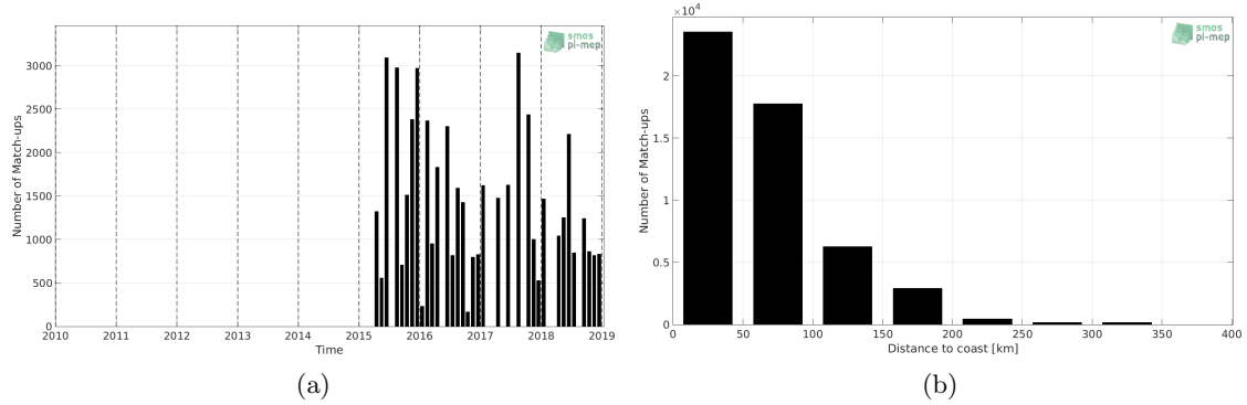
Figure 1: Number of match-ups between TSG-LEGOS-DM and SMAP-L3-RSS-V4-8DAY-RUNNING SSS as a function of time (a) and as function of the distance to coast (b) over the Mediterranean Sea Pi-MEP region and for the full satellite product period.
