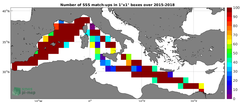
Figure 4: Number of SSS match-ups between TSG-LEGOS-DM SSS and the SMAP-L3-RSS-V4-8DAY-RUNNING SSS product for the Mediterranean Sea Pi-MEP region over 1^\circ \times 1^\circ boxes and for the full satellite product period.
