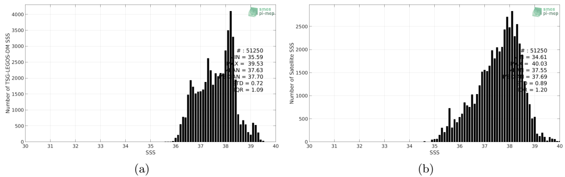
Figure 2: Histograms of SSS from TSG-LEGOS-DM (a) and SMAP-L3-RSS-V4-8DAY-RUNNING (b) considering all match-up pairs per bins of 0.1 over the Mediterranean Sea Pi-MEP region and for the full satellite product period.
