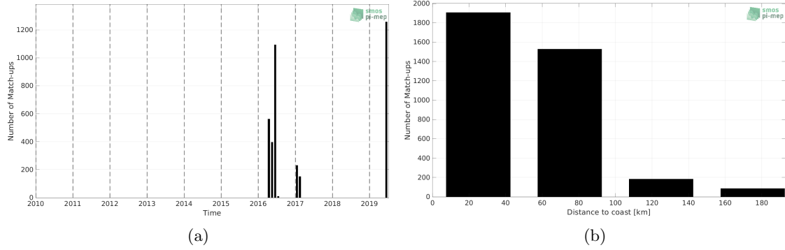
Figure 1: Number of match-ups between TSG (GOSUD-Sailing-ship) and SMAP SSS L3 v4 - 8-Day running (RSS) SSS as a function of time (a) and as function of the distance to coast (b) over the Mediterranean Sea Pi-MEP region and for the full satellite product period.
