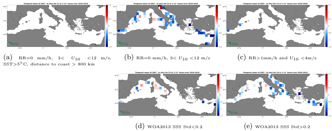
Figure 12: Temporal mean gridded over spatial boxes of size 1^\circ \times 1^\circ of \Delta\text{SSS} (SMAP SSS L3 v4 - 8-Day running (RSS) - TSG (GOSUD-Sailing-ship)) for 5 different subdatasets corresponding to:RR=0 mm/h, 3 < U_{10} < 12 m/s, SST>5°C, distance to coast > 800 km (a), RR=0 mm/h, 3 < U_{10} < 12 m/s (b), RR>1mm/h and U_{10} < 4 m/s (c), WOA2013 SSS Std<0.2 (d), WOA2013 SSS Std>0.2 (e).
