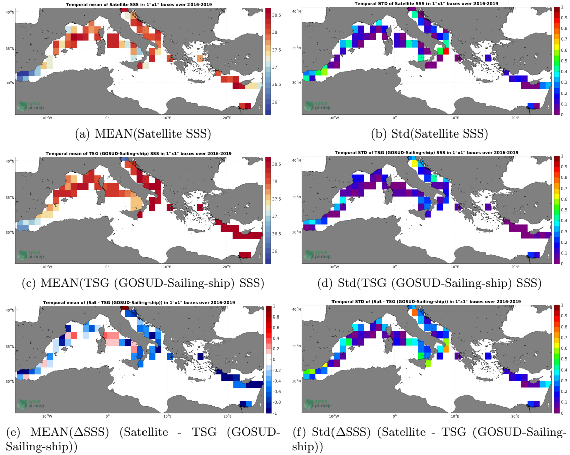
Figure 6: Temporal mean (left) and Std (right) of SSS from SMAP SSS L3 v4 - 8-Day running (RSS) (top), TSG (GOSUD-Sailing-ship) (middle), and of \Delta SSS (Satellite - TSG (GOSUD-Sailing-ship)). Only match-up pairs are used to generate these maps.
