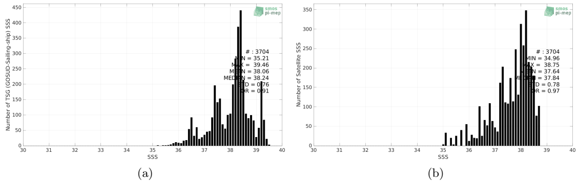
Figure 2: Histograms of SSS from TSG (GOSUD-Sailing-ship) (a) and SMAP SSS L3 v4 - 8-Day running (RSS) (b) considering all match-up pairs per bins of 0.1 over the Mediterranean Sea Pi-MEP region and for the full satellite product period.
