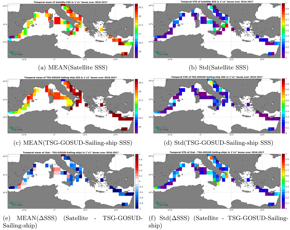
Figure 6: Temporal mean (left) and Std (right) of SSS from SMAP-L3-RSS-V4-8DAY-RUNNING (top), TSG-GOSUD-Sailing-ship (middle), and of \Delta SSS (Satellite - TSG-GOSUD-Sailing-ship). Only match-up pairs are used to generate these maps.
