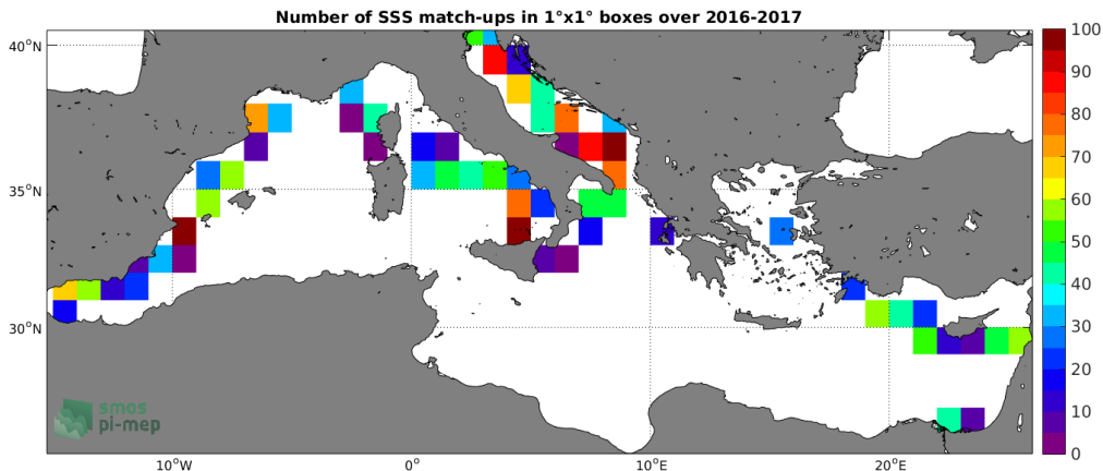
Figure 4: Number of SSS match-ups between TSG-GOSUD-Sailing-ship SSS and the SMAP-L3-RSS-V4-8DAY-RUNNING SSS product for the Mediterranean Sea Pi-MEP region over 1°x1° boxes and for the full satellite product period.
