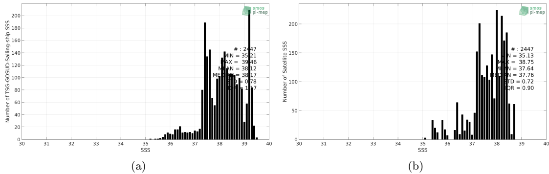
Figure 2: Histograms of SSS from TSG-GOSUD-Sailing-ship (a) and SMAP-L3-RSS-V4-8DAY-RUNNING (b) considering all match-up pairs per bins of 0.1 over the Mediterranean Sea Pi-MEP region and for the full satellite product period.
