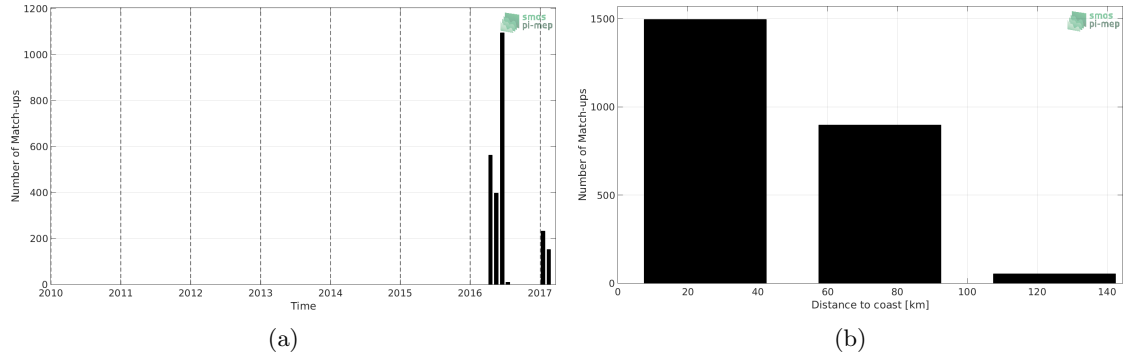
Figure 1: Number of match-ups between TSG-GOSUD-Sailing-ship and SMAP-L3-RSS-V4-8DAY-RUNNING SSS as a function of time (a) and as function of the distance to coast (b) over the Mediterranean Sea Pi-MEP region and for the full satellite product period.
