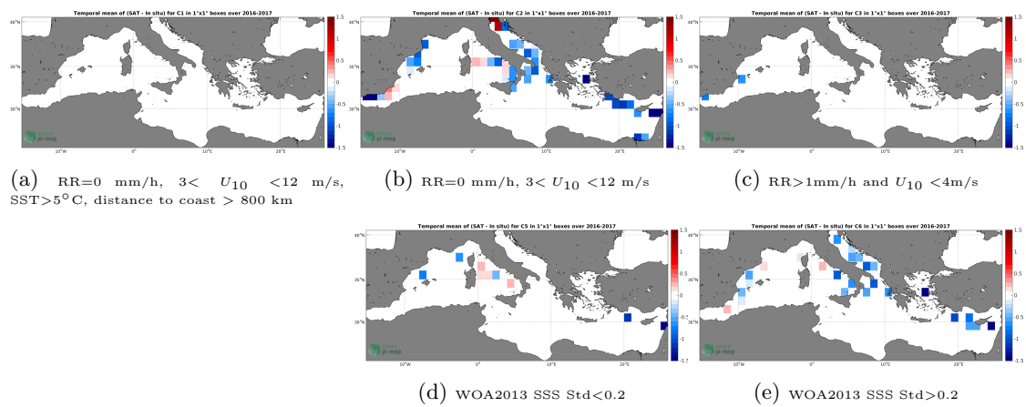
Figure 12: Temporal mean gridded over spatial boxes of size 1^\circ \times 1^\circ of \Delta SSS (SMAP-L3-RSS-V4-8DAY-RUNNING - TSG-GOSUD-Sailing-ship) for 5 different subdatasets corresponding to:RR=0 mm/h, 3 < U_{10} < 12 m/s, SST >5^\circ\text{C} , distance to coast > 800 km (a), RR=0 mm/h, 3 < U_{10} < 12 m/s (b), RR >1 mm/h and U_{10} < 4 m/s (c), WOA2013 SSS Std <0.2 (d), WOA2013 SSS Std >0.2 (e).
