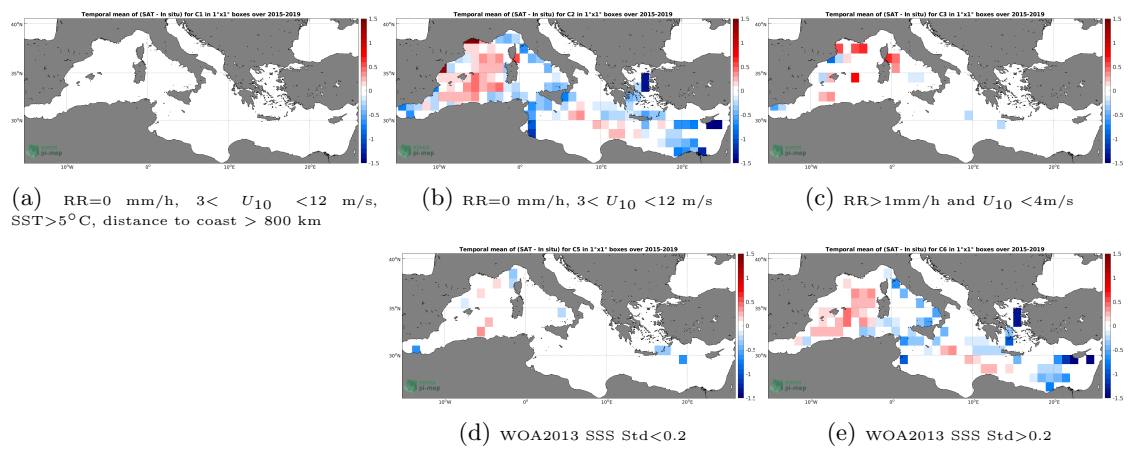
Figure 12: Temporal mean gridded over spatial boxes of size 1^\circ \times 1^\circ of \Delta SSS (SMAP SSS L3 v4 - 8-Day running (RSS) - TSG (GOSUD-Research-vessel)) for 5 different subdatasets corresponding to: RR=0 mm/h, 3 < U_{10} < 12 m/s, SST > 5°C, distance to coast > 800 km (a), RR=0 mm/h, 3 < U_{10} < 12 m/s (b), RR > 1mm/h and U_{10} < 4 m/s (c), WOA2013 SSS Std < 0.2 (d), WOA2013 SSS Std > 0.2 (e).
