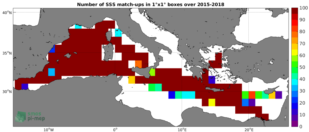
Figure 4: Number of SSS match-ups between TSG-GOSUD-Research-vessel SSS and the SMAP-L3-RSS-V4-8DAY-RUNNING SSS product for the Mediterranean Sea Pi-MEP region over 1^\circ \times 1^\circ boxes and for the full satellite product period.
