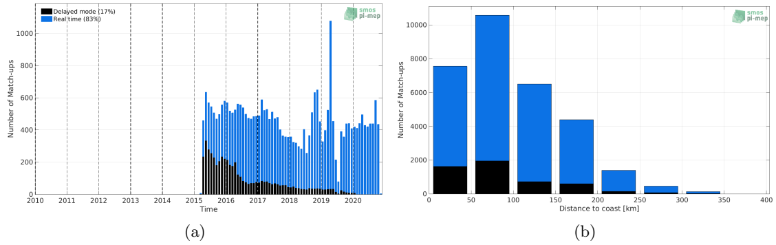
Figure 1: Number of match-ups between Argo and SMAP SSS L3 v4 - 8-Day running (RSS) SSS as a function of time (a) and as function of the distance to coast (b) over the Mediterranean Sea Pi-MEP region and for the full satellite product period.
