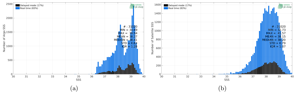
Figure 2: Histograms of SSS from Argo (a) and SMAP SSS L3 v4 - 8-Day running (RSS) (b) considering all match-up pairs per bins of 0.1 over the Mediterranean Sea Pi-MEP region and for the full satellite product period.
