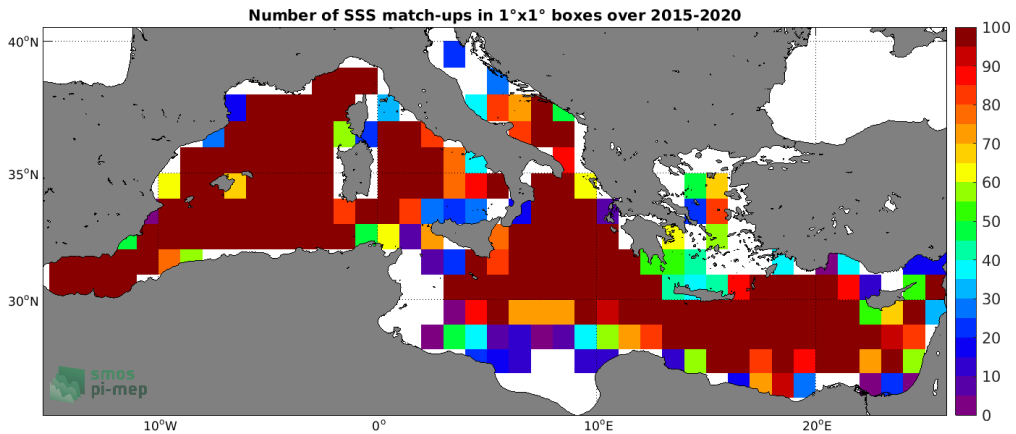
Figure 4: Number of SSS match-ups between Argo SSS and the SMAP SSS L3 v4 - 8-Day running (RSS) SSS product for the Mediterranean Sea Pi-MEP region over 1°x1° boxes and for the full satellite product period.
