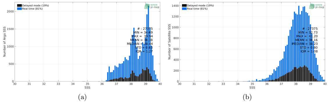
Figure 2: Histograms of SSS from Argo (a) and SMAP-L3-RSS-V4-8DAY-RUNNING (b) considering all match-up pairs per bins of 0.1 over the Mediterranean Sea Pi-MEP region and for the full satellite product period.
