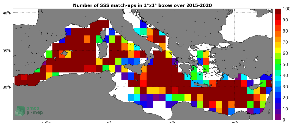
Figure 4: Number of SSS match-ups between Argo SSS and the SMAP-L3-RSS-V4-8DAY-RUNNING SSS product for the Mediterranean Sea Pi-MEP region over 1°x1° boxes and for the full satellite product period.
