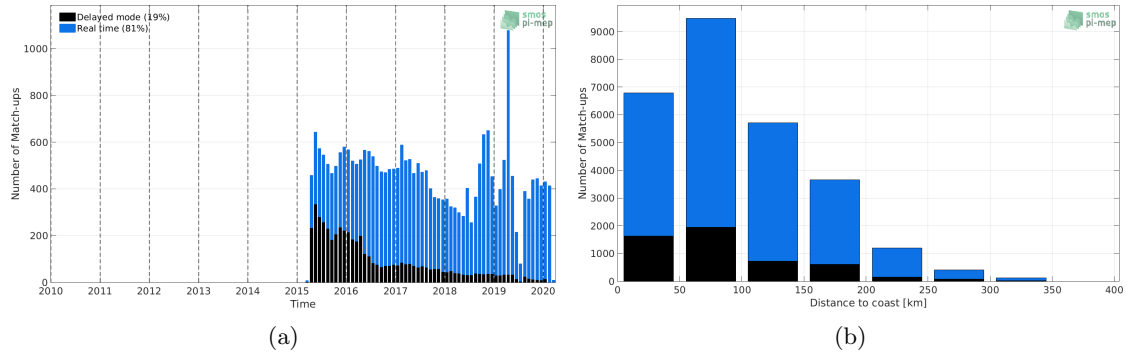
Figure 1: Number of match-ups between Argo and SMAP-L3-RSS-V4-8DAY-RUNNING SSS as a function of time (a) and as function of the distance to coast (b) over the Mediterranean Sea Pi-MEP region and for the full satellite product period.
