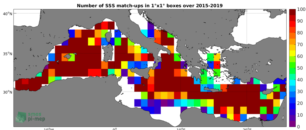
Figure 4: Number of SSS match-ups between Argo SSS and the SMAP-L3-RSS-V4-8DAY-RUNNING SSS product for the Mediterranean Sea Pi-MEP region over 1^\circ \times 1^\circ boxes and for the full satellite product period.
