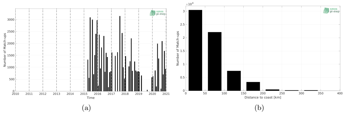
Figure 1: Number of match-ups between TSG (LEGOS-DM) and SMAP SSS L3 v4 - Monthly (RSS) SSS as a function of time (a) and as function of the distance to coast (b) over the Mediterranean Sea Pi-MEP region and for the full satellite product period.
