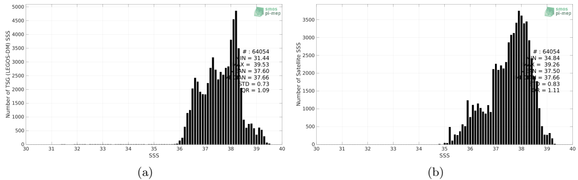
Figure 2: Histograms of SSS from TSG (LEGOS-DM) (a) and SMAP SSS L3 v4 - Monthly (RSS) (b) considering all match-up pairs per bins of 0.1 over the Mediterranean Sea Pi-MEP region and for the full satellite product period.
