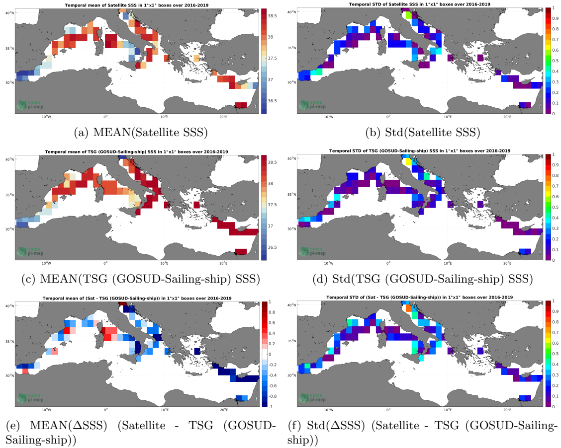
Figure 6: Temporal mean (left) and Std (right) of SSS from SMAP SSS L3 v4 - Monthly (RSS) (top), TSG (GOSUD-Sailing-ship) (middle), and of \Delta SSS (Satellite - TSG (GOSUD-Sailing-ship)). Only match-up pairs are used to generate these maps.
