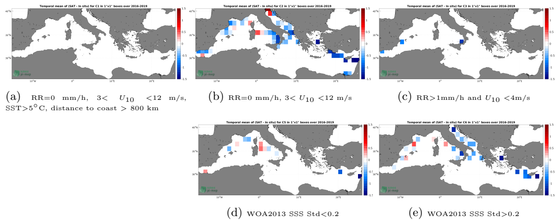
Figure 12: Temporal mean gridded over spatial boxes of size 1^\circ \times 1^\circ of \Delta\text{SSS} (SMAP SSS L3 v4 - Monthly (RSS) - TSG (GOSUD-Sailing-ship)) for 5 different subdatasets corresponding to:RR=0 mm/h, 3 < U_{10} < 12 m/s, SST>5°C, distance to coast > 800 km (a), RR=0 mm/h, 3 < U_{10} < 12 m/s (b), RR>1mm/h and U_{10} < 4 m/s (c), WOA2013 SSS Std<0.2 (d), WOA2013 SSS Std>0.2 (e).
