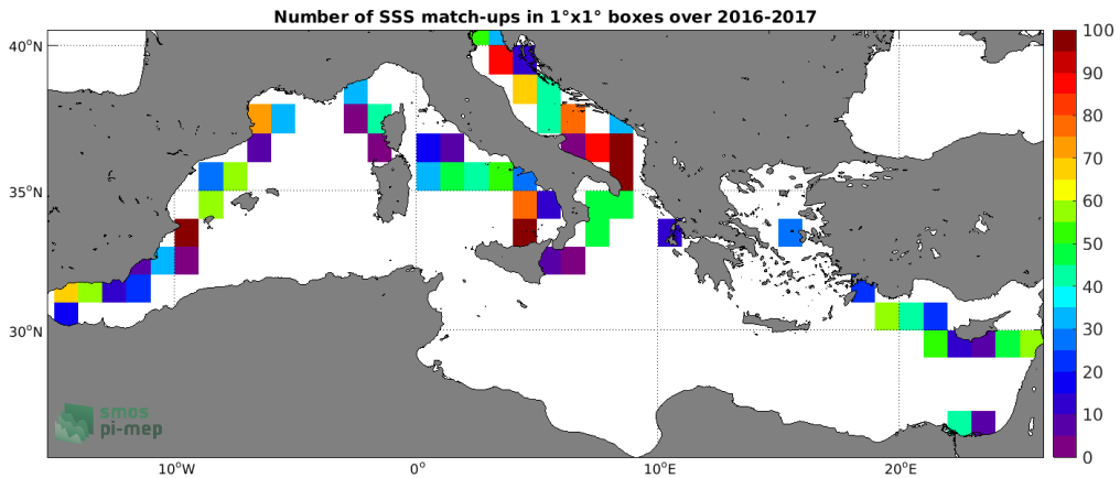
Figure 4: Number of SSS match-ups between TSG (GOSUD-Sailing-ship) SSS and the SMAP SSS L3 v4 - Monthly (RSS) SSS product for the Mediterranean Sea Pi-MEP region over 1°x1° boxes and for the full satellite product period.
