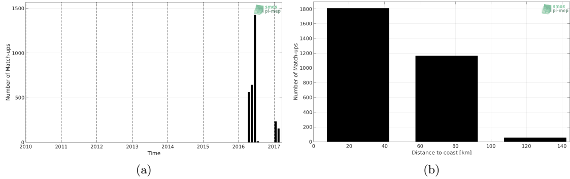
Figure 1: Number of match-ups between TSG-GOSUD-Sailing-ship and SMAP-L3-RSS-V4-MONTHLY SSS as a function of time (a) and as function of the distance to coast (b) over the Mediterranean Sea Pi-MEP region and for the full satellite product period.
