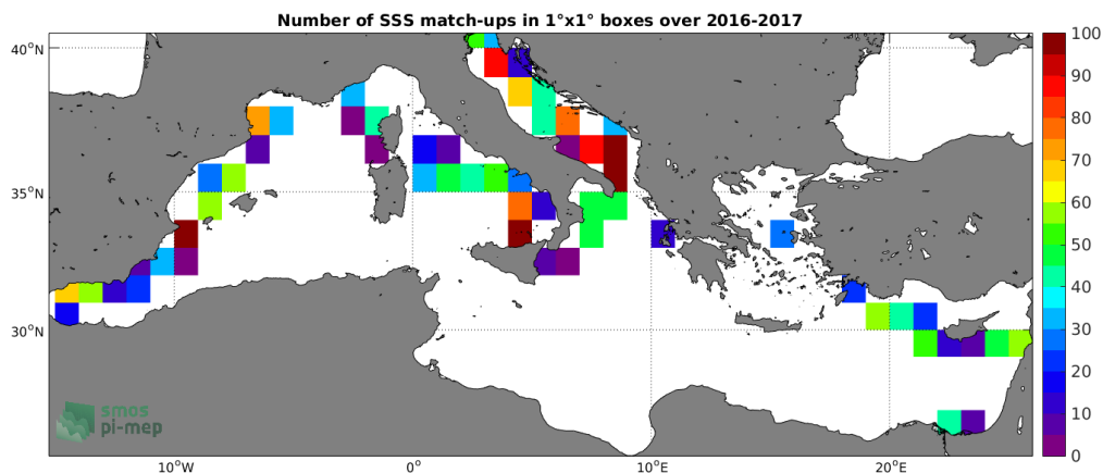
Figure 4: Number of SSS match-ups between TSG-GOSUD-Sailing-ship SSS and the SMAP-L3-RSS-V4-MONTHLY SSS product for the Mediterranean Sea Pi-MEP region over 1^\circ \times 1^\circ boxes and for the full satellite product period.
