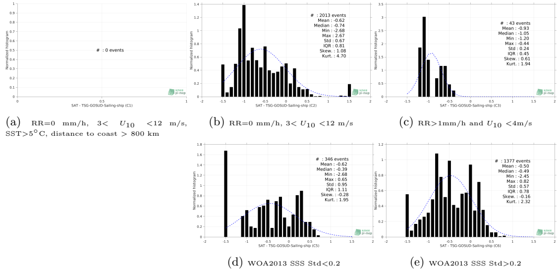
Figure 13: Normalized histogram of \Delta SSS (SMAP-L3-RSS-V4-MONTHLY - TSG-GOSUD-Sailing-ship) for 5 different subdatasets corresponding to: RR=0 mm/h, 3 < U_{10} < 12 m/s, SST > 5°C, distance to coast > 800 km (a), RR=0 mm/h, 3 < U_{10} < 12 m/s (b), RR > 1mm/h and U_{10} < 4 m/s (c), WOA2013 SSS Std < 0.2 (d), WOA2013 SSS Std > 0.2 (e).
