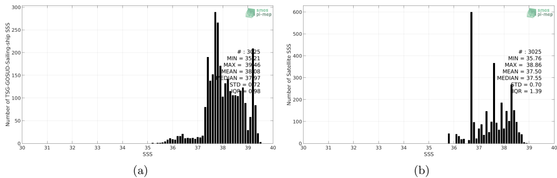
Figure 2: Histograms of SSS from TSG-GOSUD-Sailing-ship (a) and SMAP-L3-RSS-V4-MONTHLY (b) considering all match-up pairs per bins of 0.1 over the Mediterranean Sea Pi-MEP region and for the full satellite product period.
