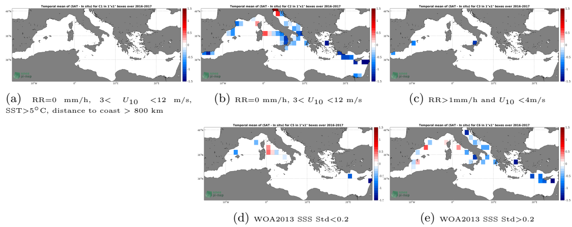
Figure 12: Temporal mean gridded over spatial boxes of size 1^\circ \times 1^\circ of \Delta SSS (SMAP-L3-RSS-V4-MONTHLY - TSG-GOSUD-Sailing-ship) for 5 different subdatasets corresponding to:RR=0 mm/h, 3 < U_{10} < 12 m/s, SST>5°C, distance to coast > 800 km (a), RR=0 mm/h, 3 < U_{10} < 12 m/s (b), RR>1mm/h and U_{10} < 4 m/s (c), WOA2013 SSS Std<0.2 (d), WOA2013 SSS Std>0.2 (e).
