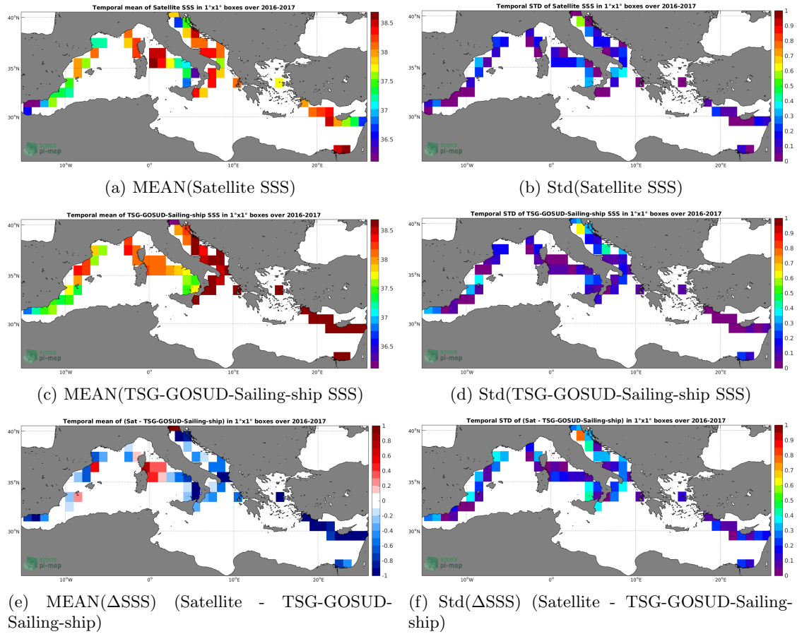
Figure 6: Temporal mean (left) and Std (right) of SSS from SMAP-L3-RSS-V4-MONTHLY (top), TSG-GOSUD-Sailing-ship (middle), and of \Delta SSS (Satellite - TSG-GOSUD-Sailing-ship). Only match-up pairs are used to generate these maps.
