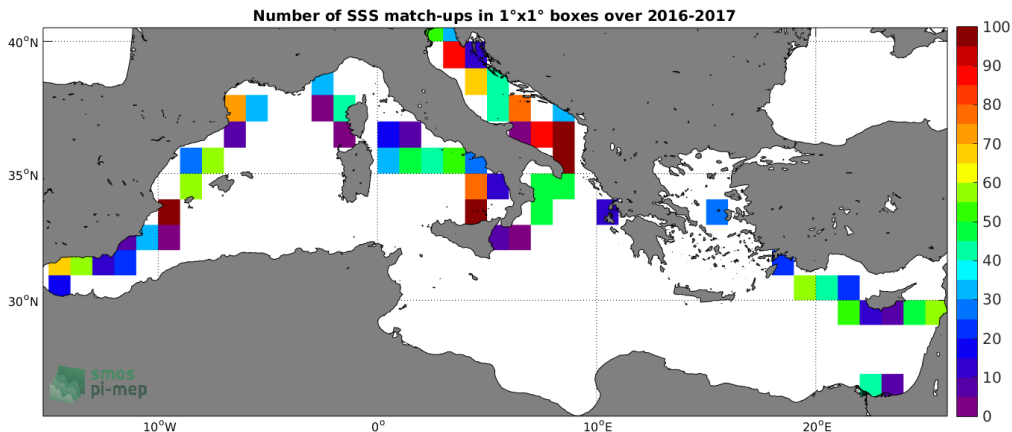
Figure 4: Number of SSS match-ups between TSG-GOSUD-Sailing-ship SSS and the SMAP-L3-RSS-V4-MONTHLY SSS product for the Mediterranean Sea Pi-MEP region over 1°x1° boxes and for the full satellite product period.
