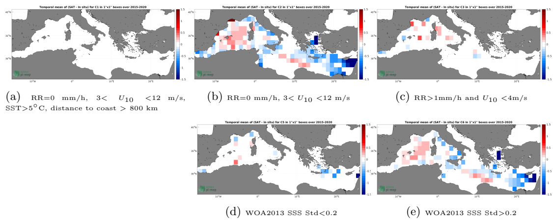
Figure 12: Temporal mean gridded over spatial boxes of size 1^\circ \times 1^\circ of \Delta SSS (SMAP SSS L3 v4 - Monthly (RSS) - TSG (GOSUD-Research-vessel)) for 5 different subdatasets corresponding to:RR=0 mm/h, 3 < U_{10} < 12 m/s, SST >5^\circ\text{C} , distance to coast > 800 km (a), RR=0 mm/h, 3 < U_{10} < 12 m/s (b), RR >1 mm/h and U_{10} < 4 m/s (c), WOA2013 SSS Std <0.2 (d), WOA2013 SSS Std >0.2 (e).
