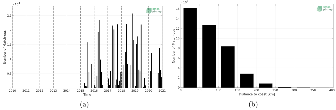
Figure 1: Number of match-ups between TSG (GOSUD-Research-vessel) and SMAP SSS L3 v4 - Monthly (RSS) SSS as a function of time (a) and as function of the distance to coast (b) over the Mediterranean Sea Pi-MEP region and for the full satellite product period.
