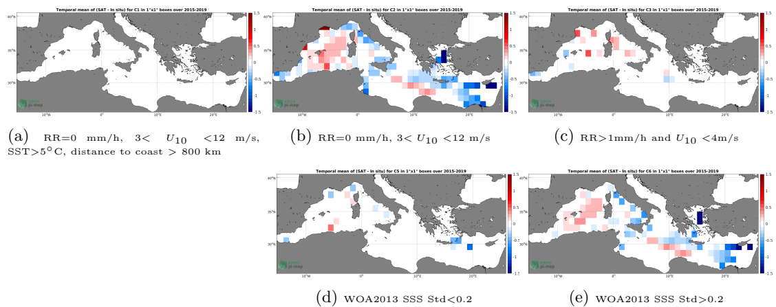
Figure 12: Temporal mean gridded over spatial boxes of size 1^\circ \times 1^\circ of \Delta SSS (SMAP SSS L3 v4 - Monthly (RSS) - TSG (GOSUD-Research-vessel)) for 5 different subdatasets corresponding to:RR=0 mm/h, 3 < U_{10} < 12 m/s, SST>5°C, distance to coast > 800 km (a), RR=0 mm/h, 3 < U_{10} < 12 m/s (b), RR>1mm/h and U_{10} < 4 m/s (c), WOA2013 SSS Std<0.2 (d), WOA2013 SSS Std>0.2 (e).
