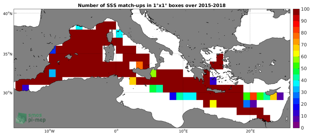
Figure 4: Number of SSS match-ups between TSG-GOSUD-Research-vessel SSS and the SMAP-L3-RSS-V4-MONTHLY SSS product for the Mediterranean Sea Pi-MEP region over 1^\circ \times 1^\circ boxes and for the full satellite product period.
