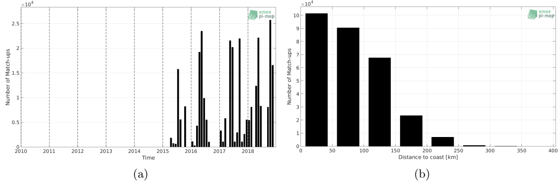
Figure 1: Number of match-ups between TSG-GOSUD-Research-vessel and SMAP-L3-RSS-V4-MONTHLY SSS as a function of time (a) and as function of the distance to coast (b) over the Mediterranean Sea Pi-MEP region and for the full satellite product period.
