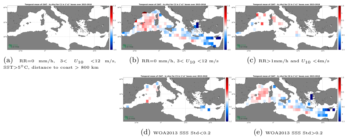
Figure 12: Temporal mean gridded over spatial boxes of size 1^\circ \times 1^\circ of \Delta SSS (SMAP-L3-RSS-V4-MONTHLY - TSG-GOSUD-Research-vessel) for 5 different subdatasets corresponding to:RR=0 mm/h, 3 < U_{10} < 12 m/s, SST>5°C, distance to coast > 800 km (a), RR=0 mm/h, 3 < U_{10} < 12 m/s (b), RR>1mm/h and U_{10} < 4 m/s (c), WOA2013 SSS Std<0.2 (d), WOA2013 SSS Std>0.2 (e).
