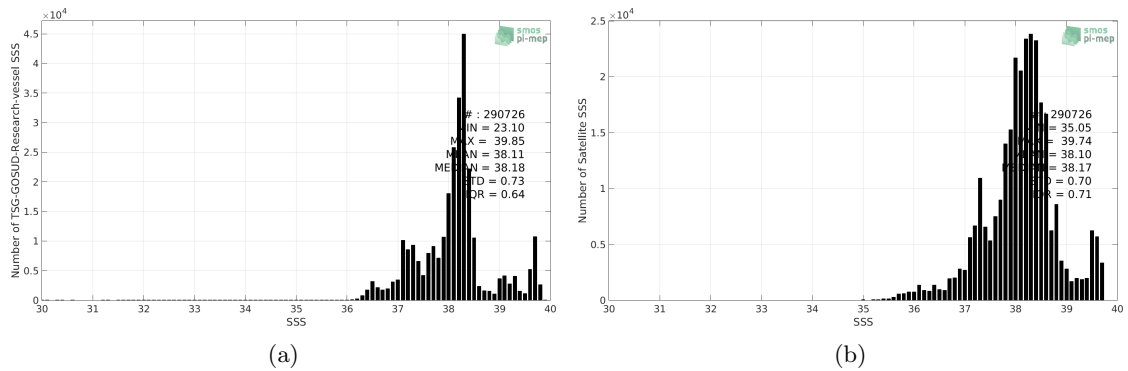
Figure 2: Histograms of SSS from TSG-GOSUD-Research-vessel (a) and SMAP-L3-RSS-V4-MONTHLY (b) considering all match-up pairs per bins of 0.1 over the Mediterranean Sea Pi-MEP region and for the full satellite product period.
