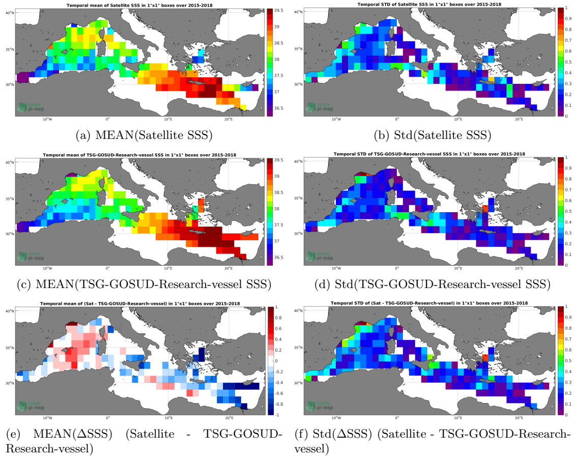
Figure 6: Temporal mean (left) and Std (right) of SSS from SMAP-L3-RSS-V4-MONTHLY (top), TSG-GOSUD-Research-vessel (middle), and of \Delta SSS (Satellite - TSG-GOSUD-Research-vessel). Only match-up pairs are used to generate these maps.
