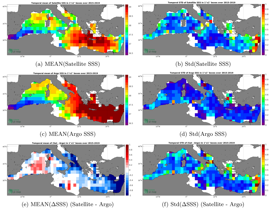
Figure 6: Temporal mean (left) and Std (right) of SSS from SMAP-L3-RSS-V4-MONTHLY (top), Argo (middle), and of \Delta SSS (Satellite - Argo). Only match-up pairs are used to generate these maps.
