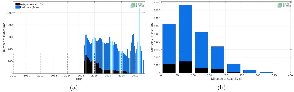
Figure 1: Number of match-ups between Argo and SMAP-L3-RSS-V4-MONTHLY SSS as a function of time (a) and as function of the distance to coast (b) over the Mediterranean Sea Pi-MEP region and for the full satellite product period.
