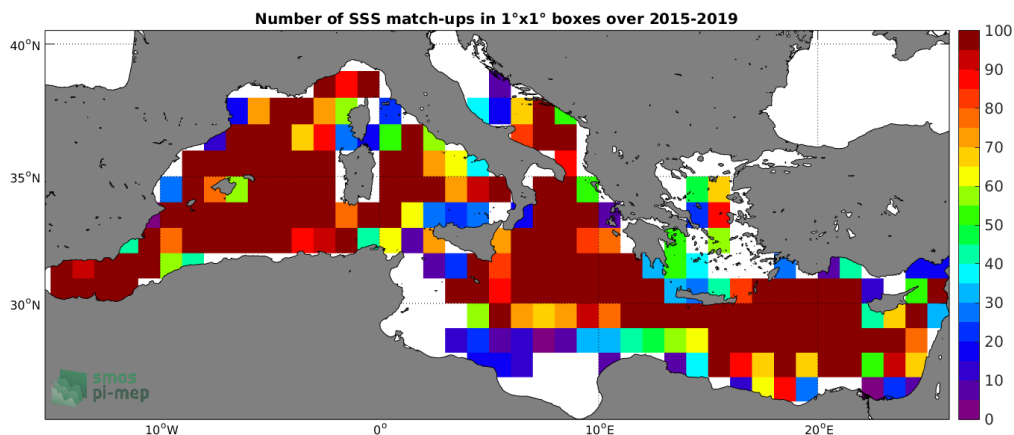
Figure 4: Number of SSS match-ups between Argo SSS and the SMAP-L3-RSS-V4-MONTHLY SSS product for the Mediterranean Sea Pi-MEP region over 1°x1° boxes and for the full satellite product period.
