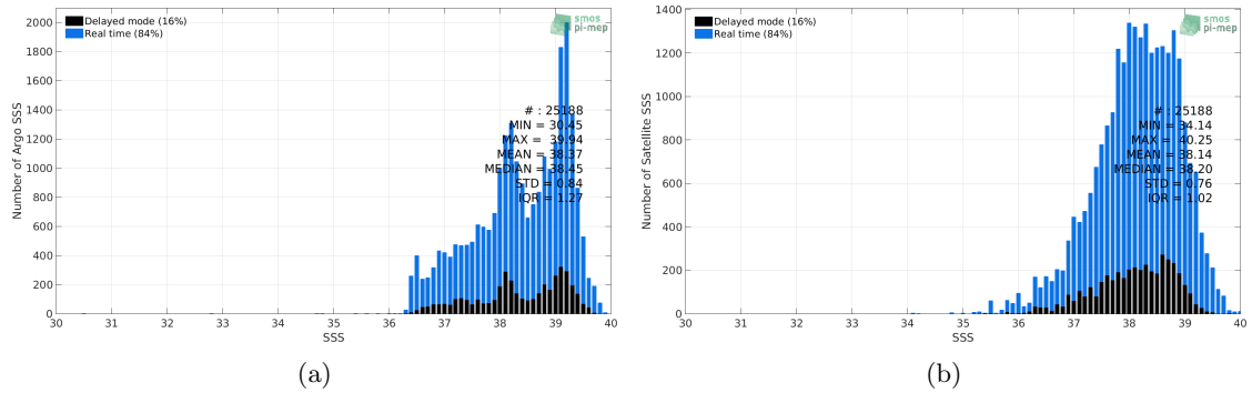
Figure 2: Histograms of SSS from Argo (a) and SMAP-L3-RSS-V4-MONTHLY (b) considering all match-up pairs per bins of 0.1 over the Mediterranean Sea Pi-MEP region and for the full satellite product period.
