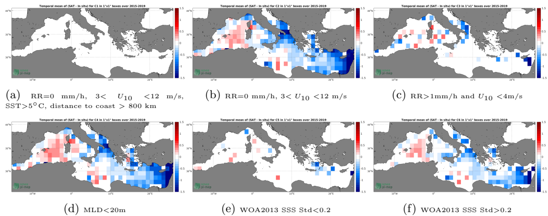
Figure 12: Temporal mean gridded over spatial boxes of size 1^\circ \times 1^\circ of \Delta SSS (SMAP-L3-RSS-V4-MONTHLY - Argo) for 6 different subdatasets corresponding to:RR=0 mm/h, 3 < U_{10} < 12 m/s, SST >5^\circ C, distance to coast > 800 km (a), RR=0 mm/h, 3 < U_{10} < 12 m/s (b), RR >1 mm/h and U_{10} < 4 m/s (c),MLD <20 m (d),WOA2013 SSS Std <0.2 (e),WOA2013 SSS Std >0.2 (f).
