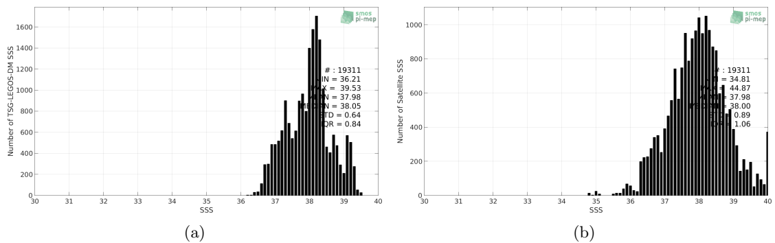
Figure 2: Histograms of SSS from TSG-LEGOS-DM (a) and SMAP-L3-RSS-V3-8DAY-RUNNING-40KM (b) considering all match-up pairs per bins of 0.1 over the Mediterranean Sea Pi-MEP region and for the full satellite product period.
