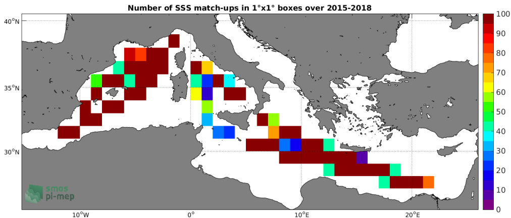
Figure 4: Number of SSS match-ups between TSG-LEGOS-DM SSS and the SMAP-L3-RSS-V3-8DAY-RUNNING-40KM SSS product for the Mediterranean Sea Pi-MEP region over 1^\circ \times 1^\circ boxes and for the full satellite product period.
