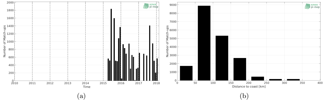
Figure 1: Number of match-ups between TSG-LEGOS-DM and SMAP-L3-RSS-V3-8DAY-RUNNING-40KM SSS as a function of time (a) and as function of the distance to coast (b) over the Mediterranean Sea Pi-MEP region and for the full satellite product period.
