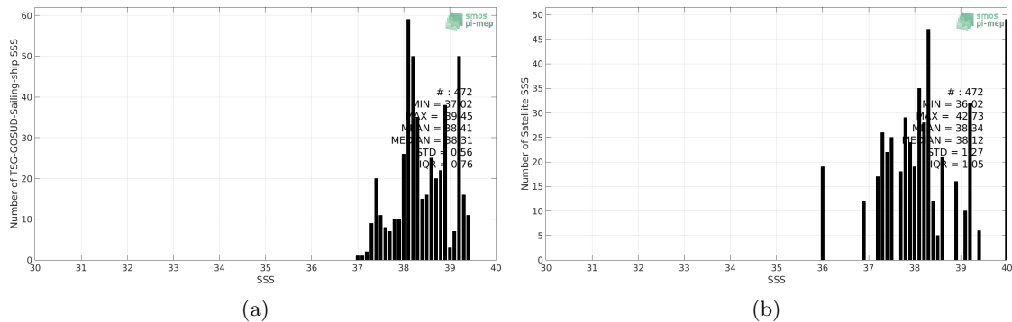
Figure 2: Histograms of SSS from TSG-GOSUD-Sailing-ship (a) and SMAP-L3-RSS-V3-8DAY-RUNNING-40KM (b) considering all match-up pairs per bins of 0.1 over the Mediterranean Sea Pi-MEP region and for the full satellite product period.
