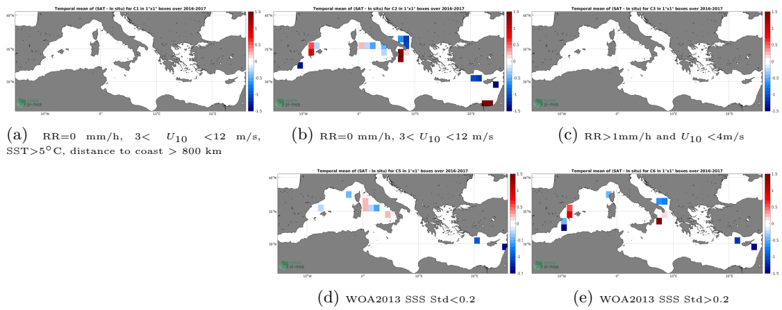
Figure 12: Temporal mean gridded over spatial boxes of size 1^\circ \times 1^\circ of \Delta SSS (SMAP-L3-RSS-V3-8DAY-RUNNING-40KM - TSG-GOSUD-Sailing-ship) for 5 different subdatasets corresponding to:RR=0 mm/h, 3 < U_{10} < 12 m/s, SST >5^\circ\text{C} , distance to coast > 800 km (a), RR=0 mm/h, 3 < U_{10} < 12 m/s (b), RR >1 mm/h and U_{10} < 4 m/s (c), WOA2013 SSS Std <0.2 (d), WOA2013 SSS Std >0.2 (e).
