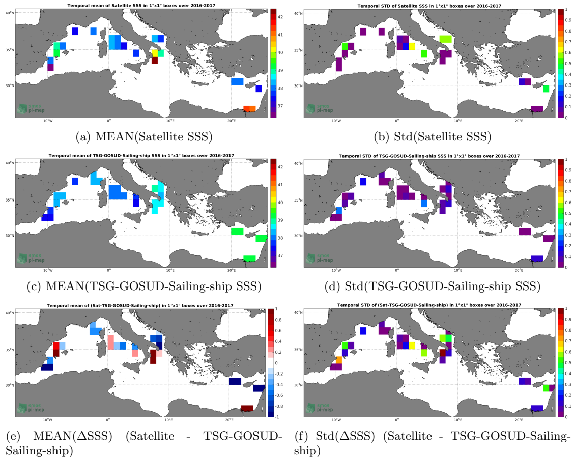
Figure 6: Temporal mean (left) and Std (right) of SSS from SMAP-L3-RSS-V3-8DAY-RUNNING-40KM (top), TSG-GOSUD-Sailing-ship (middle), and of \Delta SSS (Satellite - TSG-GOSUD-Sailing-ship). Only match-up pairs are used to generate these maps.
