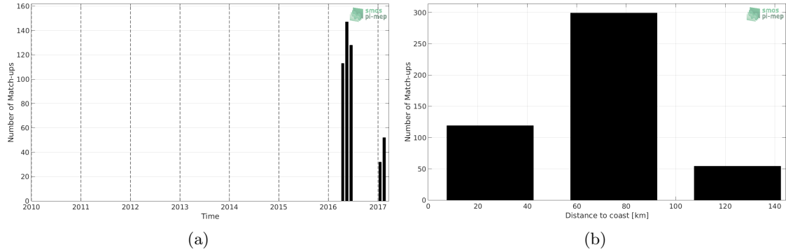
Figure 1: Number of match-ups between TSG-GOSUD-Sailing-ship and SMAP-L3-RSS-V3-8DAY-RUNNING-40KM SSS as a function of time (a) and as function of the distance to coast (b) over the Mediterranean Sea Pi-MEP region and for the full satellite product period.
