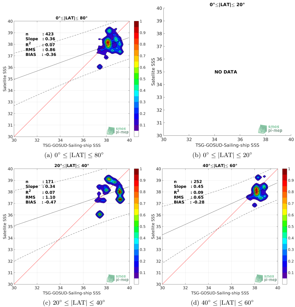
Figure 9: Contour maps of the concentration of SMAP-L3-RSS-V3-8DAY-RUNNING-40KM SSS (y-axis) versus TSG-GOSUD-Sailing-ship SSS (x-axis) at match-up pairs for different latitude bands. For each plot, the red line shows x=y . The black thin and dashed lines indicate a linear fit through the data cloud and the \pm 95\% confidence levels, respectively. The number match-up pairs n , the slope and R^2 coefficient of the linear fit, the root mean square (RMS) and the mean bias between satellite and in situ data are indicated for each latitude band in each plots.
