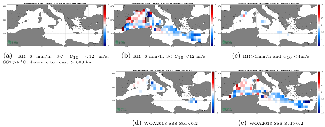
Figure 12: Temporal mean gridded over spatial boxes of size 1^\circ \times 1^\circ of \Delta SSS (SMAP-L3-RSS-V3-8DAY-RUNNING-40KM - TSG-GOSUD-Research-vessel) for 5 different subdatasets corresponding to:RR=0 mm/h, 3 < U_{10} < 12 m/s, SST >5^\circ C, distance to coast > 800 km (a), RR=0 mm/h, 3 < U_{10} < 12 m/s (b), RR >1 mm/h and U_{10} < 4 m/s (c), WOA2013 SSS Std <0.2 (d), WOA2013 SSS Std >0.2 (e).
