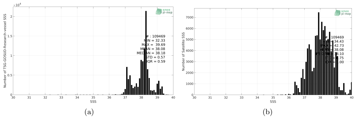
Figure 2: Histograms of SSS from TSG-GOSUD-Research-vessel (a) and SMAP-L3-RSS-V3-8DAY-RUNNING-40KM (b) considering all match-up pairs per bins of 0.1 over the Mediterranean Sea Pi-MEP region and for the full satellite product period.
