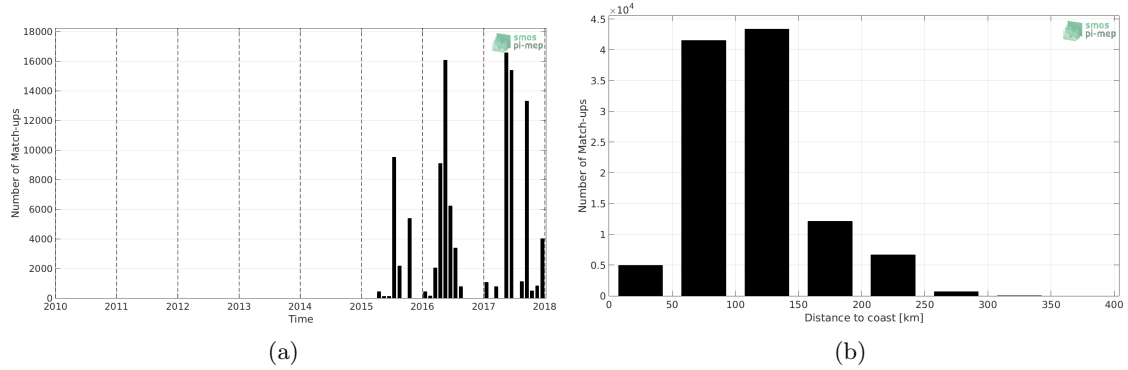
Figure 1: Number of match-ups between TSG-GOSUD-Research-vessel and SMAP-L3-RSS-V3-8DAY-RUNNING-40KM SSS as a function of time (a) and as function of the distance to coast (b) over the Mediterranean Sea Pi-MEP region and for the full satellite product period.
