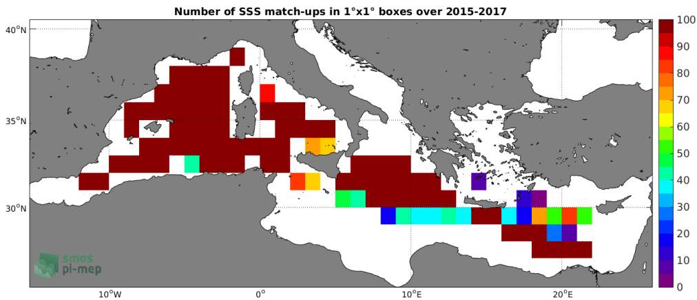
Figure 4: Number of SSS match-ups between TSG-GOSUD-Research-vessel SSS and the SMAP-L3-RSS-V3-8DAY-RUNNING-40KM SSS product for the Mediterranean Sea Pi-MEP region over 1^\circ \times 1^\circ boxes and for the full satellite product period.
