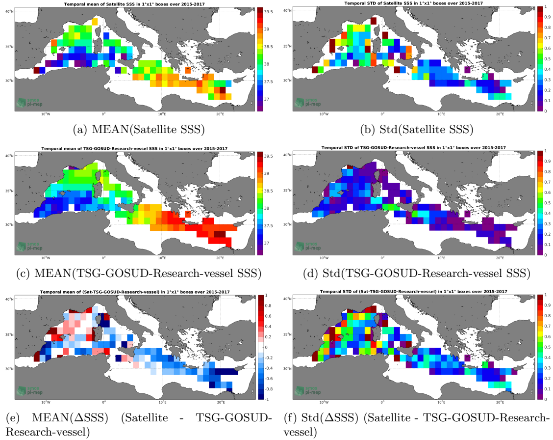
Figure 6: Temporal mean (left) and Std (right) of SSS from SMAP-L3-RSS-V3-8DAY-RUNNING-40KM (top), TSG-GOSUD-Research-vessel (middle), and of \Delta SSS (Satellite - TSG-GOSUD-Research-vessel). Only match-up pairs are used to generate these maps.
