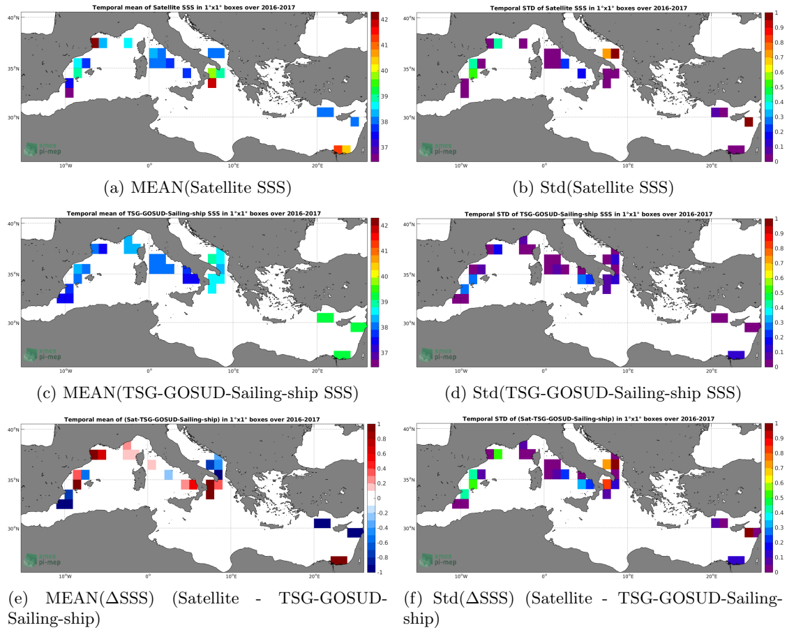
Figure 6: Temporal mean (left) and Std (right) of SSS from SMAP-L3-RSS-V3-MONTHLY-0.25DEG-40KM (top), TSG-GOSUD-Sailing-ship (middle), and of \Delta SSS (Satellite - TSG-GOSUD-Sailing-ship). Only match-up pairs are used to generate these maps.
