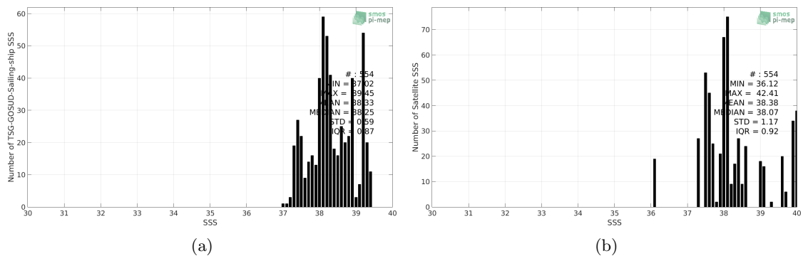
Figure 2: Histograms of SSS from TSG-GOSUD-Sailing-ship (a) and SMAP-L3-RSS-V3-MONTHLY-0.25DEG-40KM (b) considering all match-up pairs per bins of 0.1 over the Mediterranean Sea Pi-MEP region and for the full satellite product period.
