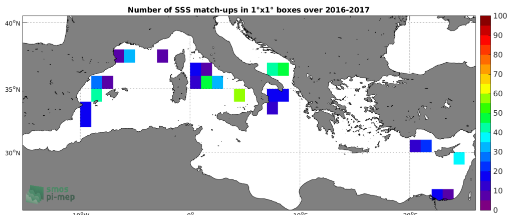
Figure 4: Number of SSS match-ups between TSG-GOSUD-Sailing-ship SSS and the SMAP-L3-RSS-V3-MONTHLY-0.25DEG-40KM SSS product for the Mediterranean Sea Pi-MEP region over 1^\circ \times 1^\circ boxes and for the full satellite product period.
