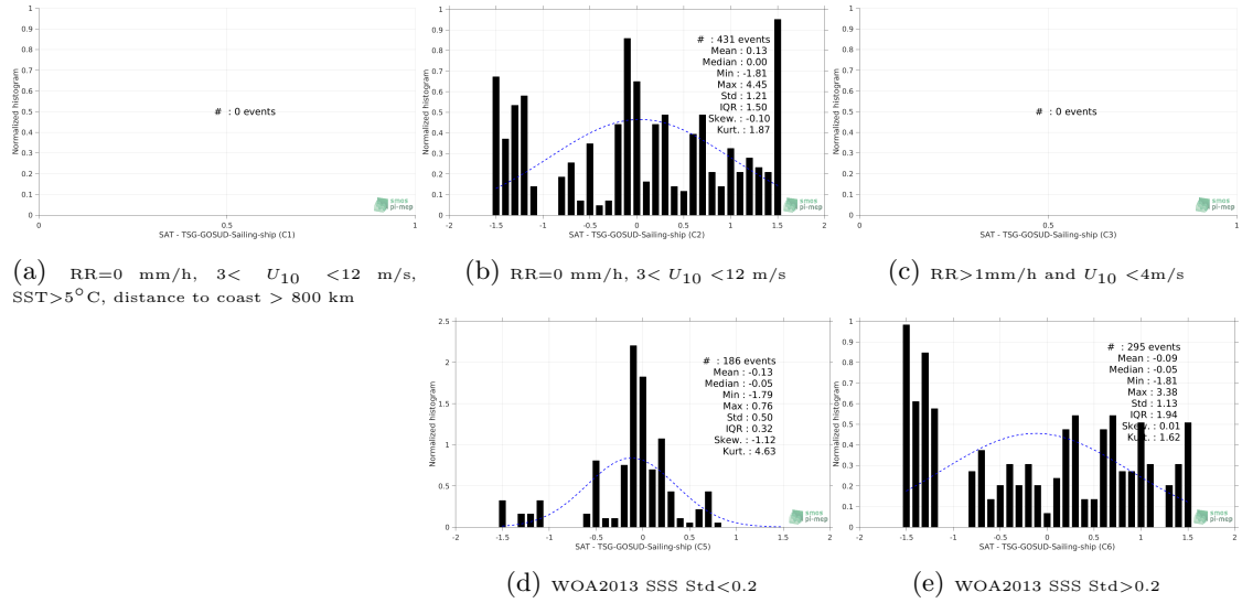
Figure 13: Normalized histogram of \Delta SSS (SMAP-L3-RSS-V3-MONTHLY-0.25DEG-40KM - TSG-GOSUD-Sailing-ship) for 5 different subdatasets corresponding to: RR=0 mm/h, 3 < U_{10} < 12 m/s, SST>5°C, distance to coast > 800 km (a), RR=0 mm/h, 3 < U_{10} < 12 m/s (b), RR>1mm/h and U_{10} < 4 m/s (c), WOA2013 SSS Std<0.2 (d), WOA2013 SSS Std>0.2 (e).
