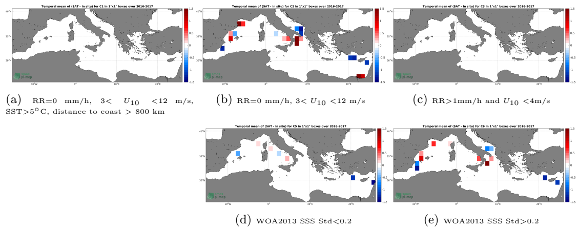
Figure 12: Temporal mean gridded over spatial boxes of size 1^\circ \times 1^\circ of \Delta SSS (SMAP-L3-RSS-V3-MONTHLY-0.25DEG-40KM - TSG-GOSUD-Sailing-ship) for 5 different subdatasets corresponding to:RR=0 mm/h, 3 < U_{10} < 12 m/s, SST >5^\circ C, distance to coast > 800 km (a), RR=0 mm/h, 3 < U_{10} < 12 m/s (b), RR >1 mm/h and U_{10} < 4 m/s (c), WOA2013 SSS Std <0.2 (d), WOA2013 SSS Std >0.2 (e).
