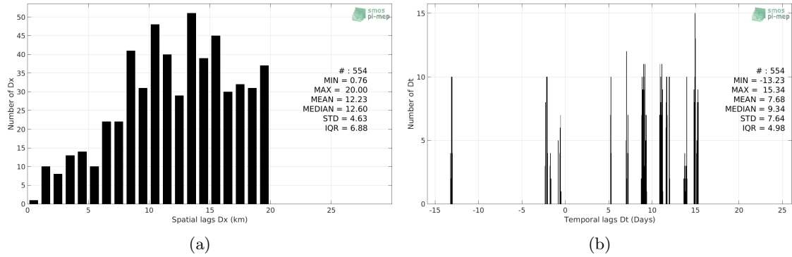
Figure 5: Histograms of the spatial (a) and temporal (b) lags between the time of the TSG-GOSUD-Sailing-ship measurements and the date of the corresponding SMAP-L3-RSS-V3-MONTHLY-0.25DEG-40KM SSS product.
