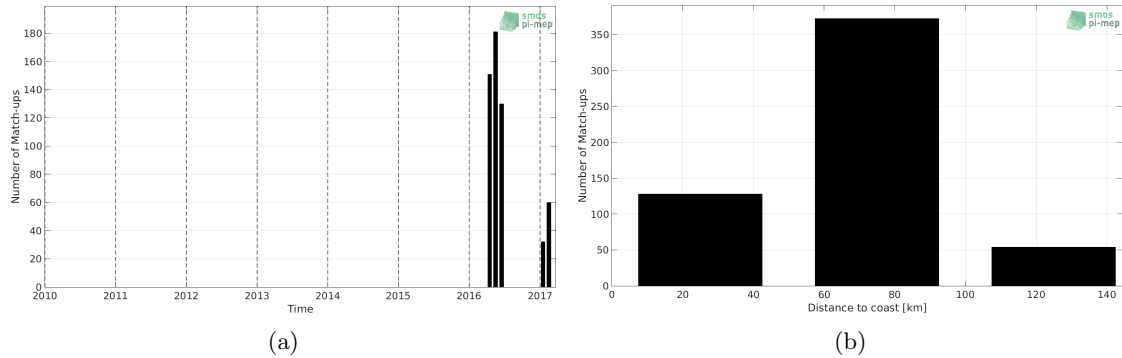
Figure 1: Number of match-ups between TSG-GOSUD-Sailing-ship and SMAP-L3-RSS-V3-MONTHLY-0.25DEG-40KM SSS as a function of time (a) and as function of the distance to coast (b) over the Mediterranean Sea Pi-MEP region and for the full satellite product period.
