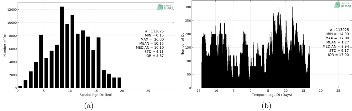
Figure 5: Histograms of the spatial (a) and temporal (b) lags between the time of the TSG-GOSUD-Research-vessel measurements and the date of the corresponding SMAP-L3-RSS-V3-MONTHLY-0.25DEG-40KM SSS product.
