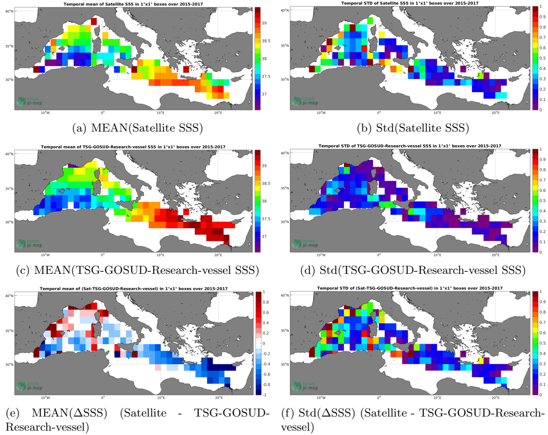
Figure 6: Temporal mean (left) and Std (right) of SSS from SMAP-L3-RSS-V3-MONTHLY-0.25DEG-40KM (top), TSG-GOSUD-Research-vessel (middle), and of \Delta SSS (Satellite - TSG-GOSUD-Research-vessel). Only match-up pairs are used to generate these maps.
