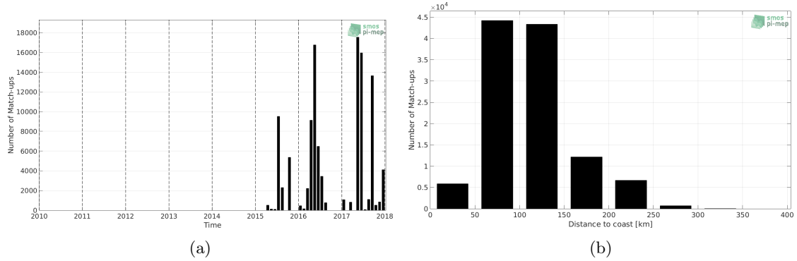
Figure 1: Number of match-ups between TSG-GOSUD-Research-vessel and SMAP-L3-RSS-V3-MONTHLY-0.25DEG-40KM SSS as a function of time (a) and as function of the distance to coast (b) over the Mediterranean Sea Pi-MEP region and for the full satellite product period.
