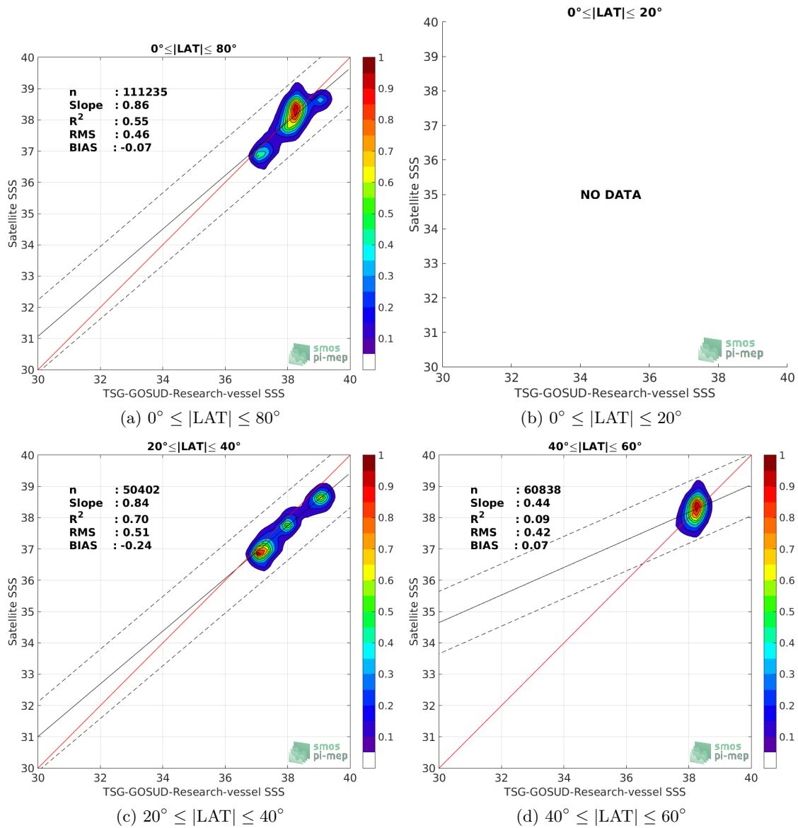
Figure 9: Contour maps of the concentration of SMAP-L3-RSS-V3-MONTHLY-0.25DEG-40KM SSS (y-axis) versus TSG-GOSUD-Research-vessel SSS (x-axis) at match-up pairs for different latitude bands. For each plot, the red line shows x=y . The black thin and dashed lines indicate a linear fit through the data cloud and the \pm 95\% confidence levels, respectively. The number match-up pairs n , the slope and R^2 coefficient of the linear fit, the root mean square (RMS) and the mean bias between satellite and in situ data are indicated for each latitude band in each plots.
