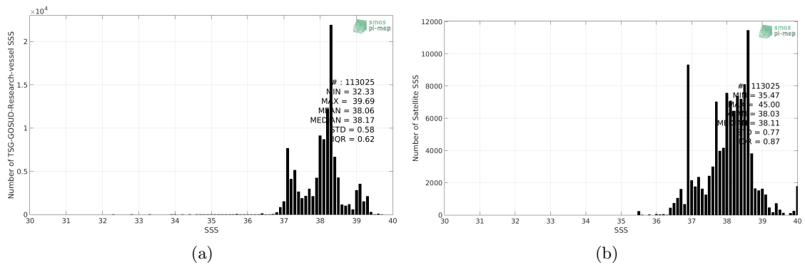
Figure 2: Histograms of SSS from TSG-GOSUD-Research-vessel (a) and SMAP-L3-RSS-V3-MONTHLY-0.25DEG-40KM (b) considering all match-up pairs per bins of 0.1 over the Mediterranean Sea Pi-MEP region and for the full satellite product period.
