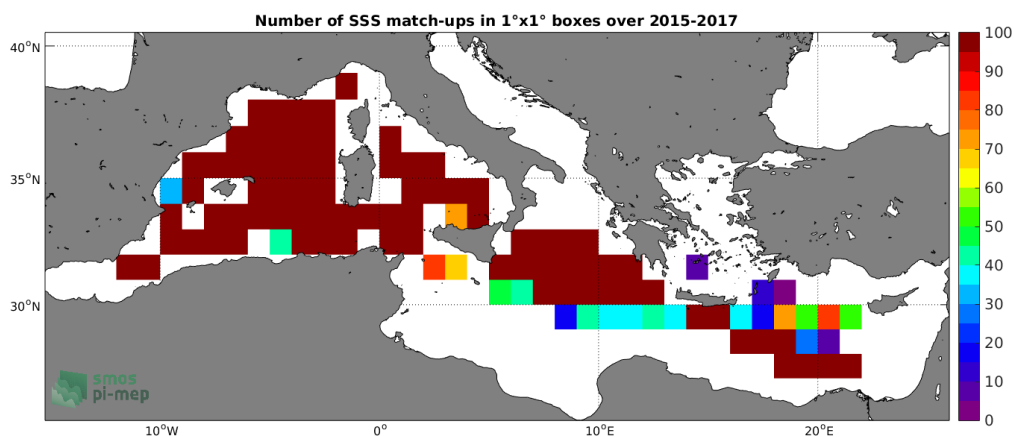
Figure 4: Number of SSS match-ups between TSG-GOSUD-Research-vessel SSS and the SMAP-L3-RSS-V3-MONTHLY-0.25DEG-40KM SSS product for the Mediterranean Sea Pi-MEP region over 1^\circ \times 1^\circ boxes and for the full satellite product period.
