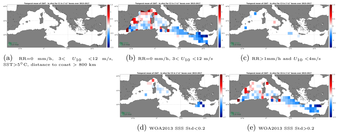
Figure 12: Temporal mean gridded over spatial boxes of size 1^\circ \times 1^\circ of \Delta SSS (SMAP-L3-RSS-V3-MONTHLY-0.25DEG-40KM - TSG-GOSUD-Research-vessel) for 5 different subdatasets corresponding to:RR=0 mm/h, 3 < U_{10} < 12 m/s, SST >5^\circ C, distance to coast > 800 km (a), RR=0 mm/h, 3 < U_{10} < 12 m/s (b), RR >1 mm/h and U_{10} < 4 m/s (c), WOA2013 SSS Std <0.2 (d), WOA2013 SSS Std >0.2 (e).
