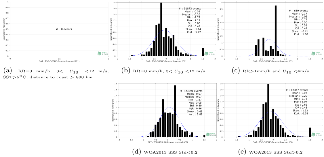
Figure 13: Normalized histogram of \Delta SSS (SMAP-L3-RSS-V3-MONTHLY-0.25DEG-40KM - TSG-GOSUD-Research-vessel) for 5 different subdatasets corresponding to: RR=0 mm/h, 3 < U_{10} < 12 m/s, SST > 5°C, distance to coast > 800 km (a), RR=0 mm/h, 3 < U_{10} < 12 m/s (b), RR > 1mm/h and U_{10} < 4 m/s (c), WOA2013 SSS Std < 0.2 (d), WOA2013 SSS Std > 0.2 (e).
