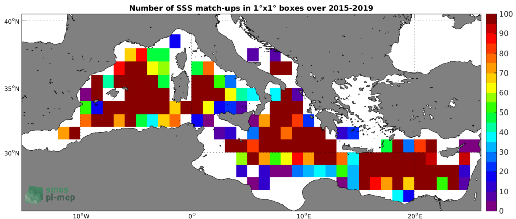
Figure 4: Number of SSS match-ups between Argo SSS and the SMAP-L3-RSS-V3-MONTHLY-0.25DEG-40KM SSS product for the Mediterranean Sea Pi-MEP region over 1^\circ \times 1^\circ boxes and for the full satellite product period.
