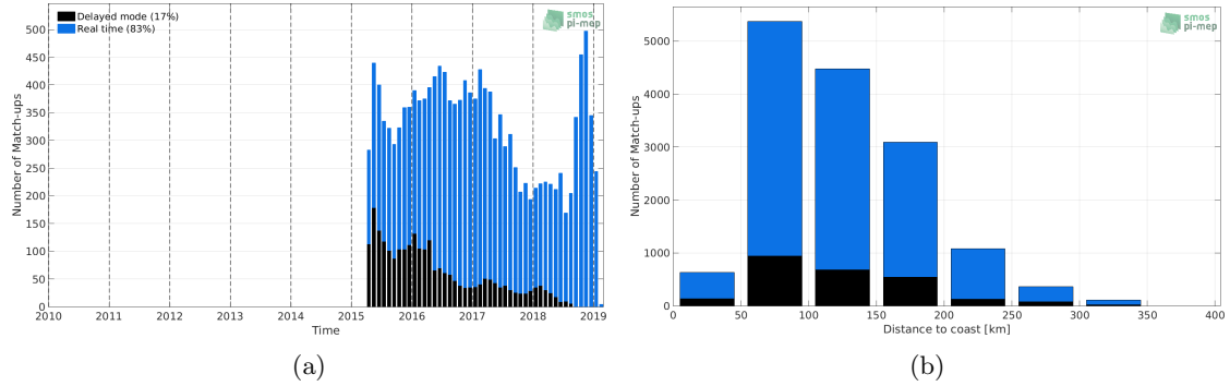
Figure 1: Number of match-ups between Argo and SMAP-L3-RSS-V3-MONTHLY-0.25DEG-40KM SSS as a function of time (a) and as function of the distance to coast (b) over the Mediterranean Sea Pi-MEP region and for the full satellite product period.
