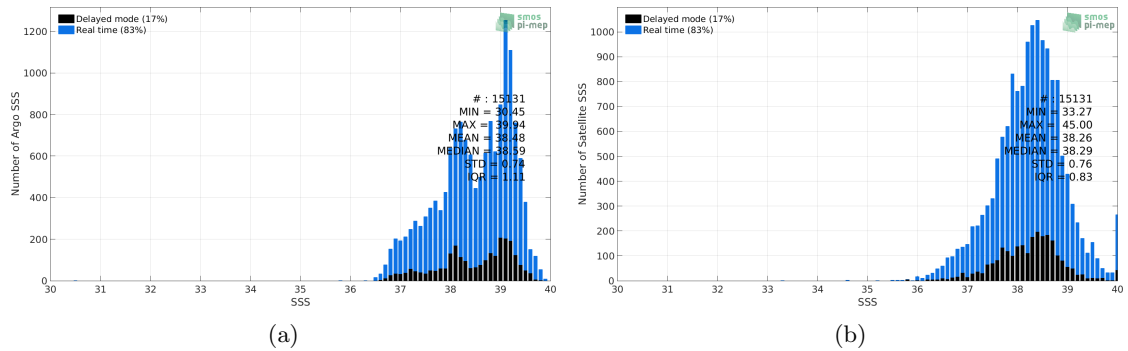
Figure 2: Histograms of SSS from Argo (a) and SMAP-L3-RSS-V3-MONTHLY-0.25DEG-40KM (b) considering all match-up pairs per bins of 0.1 over the Mediterranean Sea Pi-MEP region and for the full satellite product period.
