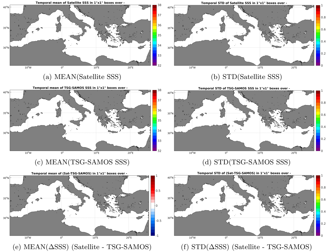
Figure 6: Temporal mean (left) and STD (right) of SSS from SMAP-L3-RSS-V2-8DAY-RUNNING-40KM (top), TSG-SAMOS (middle), and of \Delta SSS (Satellite - TSG-SAMOS). Only match-up pairs are used to generate these maps.
