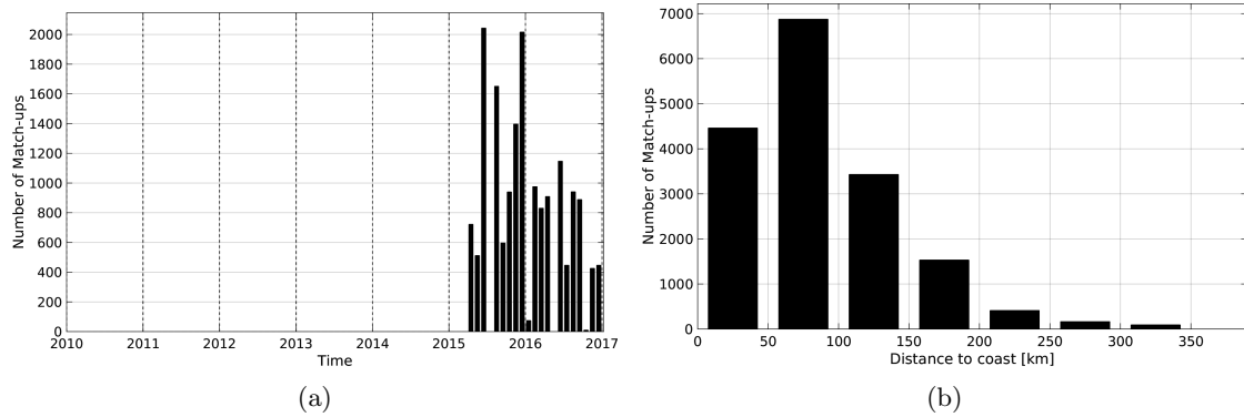
Figure 1: Number of match-ups between TSG-LEGOS-DM and SMAP-L3-RSS-V2-8DAY-RUNNING-40KM SSS as a function of time (a) and as function of the distance to coast (b) over the Mediterranean Sea Pi-MEP region and for the full satellite product period.
