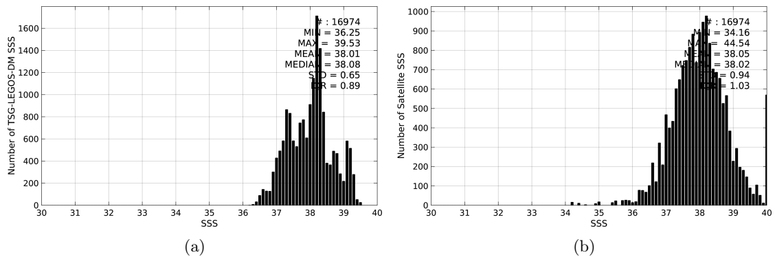
Figure 2: Histograms of SSS from TSG-LEGOS-DM (a) and SMAP-L3-RSS-V2-8DAY-RUNNING-40KM (b) considering all match-up pairs per bins of 0.1 over the Mediterranean Sea Pi-MEP region and for the full satellite product period.
