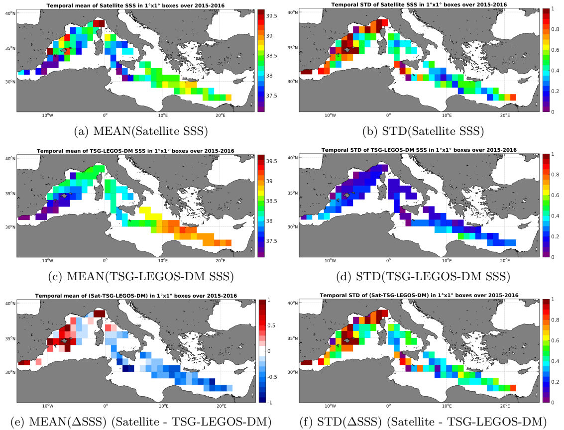
Figure 6: Temporal mean (left) and STD (right) of SSS from SMAP-L3-RSS-V2-8DAY-RUNNING-40KM (top), TSG-LEGOS-DM (middle), and of \Delta SSS (Satellite - TSG-LEGOS-DM). Only match-up pairs are used to generate these maps.
