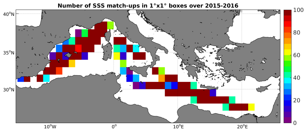
Figure 4: Number of SSS match-ups between TSG-LEGOS-DM SSS and the SMAP-L3-RSS-V2-8DAY-RUNNING-40KM SSS product for the Mediterranean Sea Pi-MEP region over 1^\circ \times 1^\circ boxes and for the full satellite product period.
