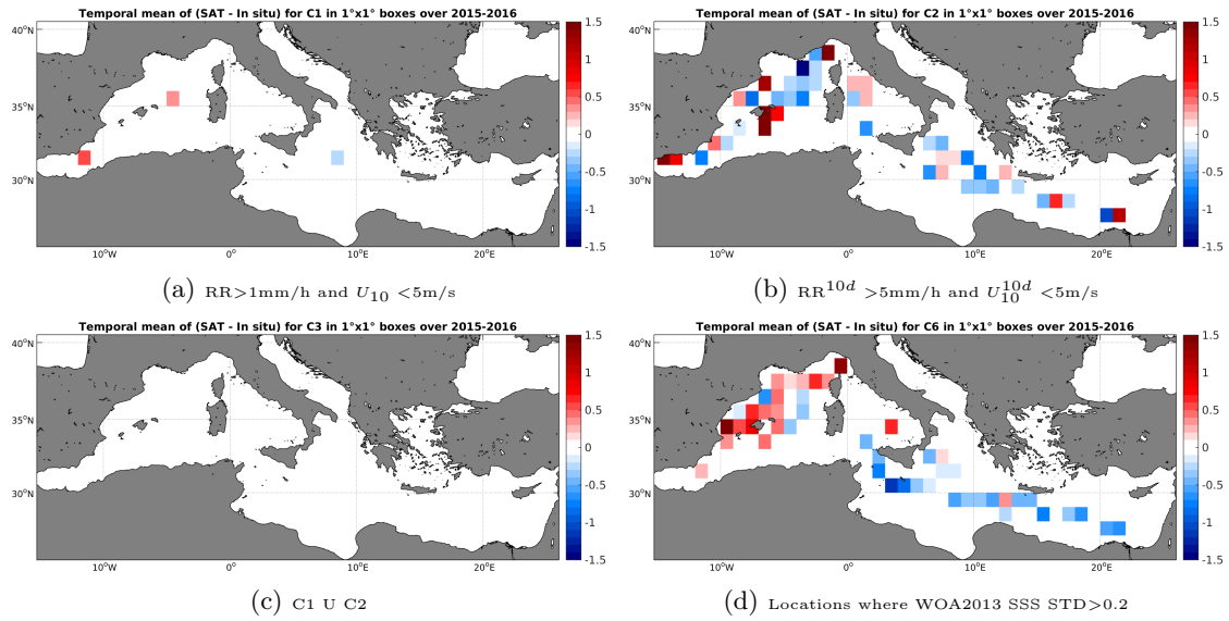
Figure 12: Temporal mean gridded over spatial boxes of size 1^\circ \times 1^\circ of \Delta SSS (SMAP-L3-RSS-V2-8DAY-RUNNING-40KM - TSG-LEGOS-DM) for 4 different subdatasets corresponding to: RR > 1\text{mm/h} and U_{10} < 5\text{m/s} (a), RR^{10d} > 5\text{mm/h} and U_{10}^{10d} < 5\text{m/s} (b), C1 U C2 (c), Locations where WOA2013 SSS STD > 0.2 (d).
