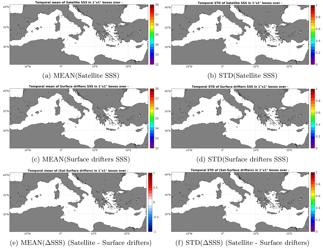
Figure 5: Temporal mean (left) and STD (right) of SSS from SMAP-L3-RSS-V2-8DAY-RUNNING-40KM (top), Surface drifters (middle), and of \Delta SSS (Satellite - Surface drifters). Only match-up pairs are used to generate these maps.
