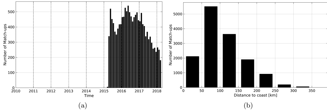
Figure 1: Number of match-ups between Argo and SMAP-L3-RSS-V2-8DAY-RUNNING-40KM SSS as a function of time (a) and as function of the distance to coast (b) over the Mediterranean Sea Pi-MEP region and for the full satellite product period.
