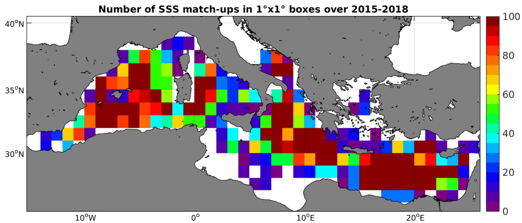
Figure 4: Number of SSS match-ups between Argo SSS and the SMAP-L3-RSS-V2-8DAY-RUNNING-40KM SSS product for the Mediterranean Sea Pi-MEP region over 1^\circ \times 1^\circ boxes and for the full satellite product period.
