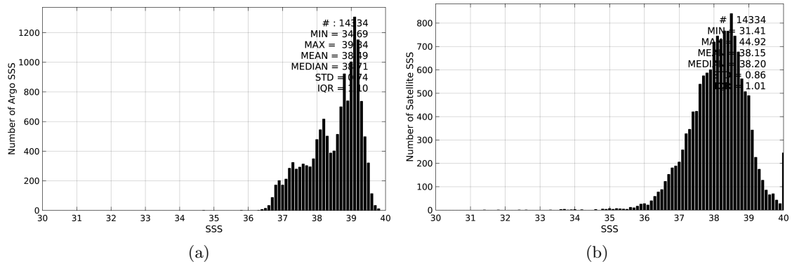
Figure 2: Histograms of SSS from Argo (a) and SMAP-L3-RSS-V2-8DAY-RUNNING-40KM (b) considering all match-up pairs per bins of 0.1 over the Mediterranean Sea Pi-MEP region and for the full satellite product period.
