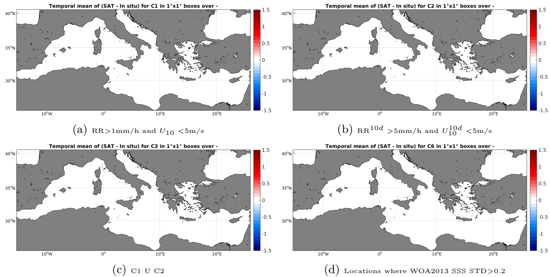
Figure 12: Temporal mean gridded over spatial boxes of size 1^\circ \times 1^\circ of \Delta SSS (SMAP-L3-RSS-V2-8DAY-RUNNING-70KM - TSG-SAMOS) for 4 different subdatasets corresponding to: RR > 1\text{mm/h} and U_{10} < 5\text{m/s} (a), RR^{10d} > 5\text{mm/h} and U_{10}^{10d} < 5\text{m/s} (b), C1 U C2 (c), Locations where WOA2013 SSS STD > 0.2 (d).
