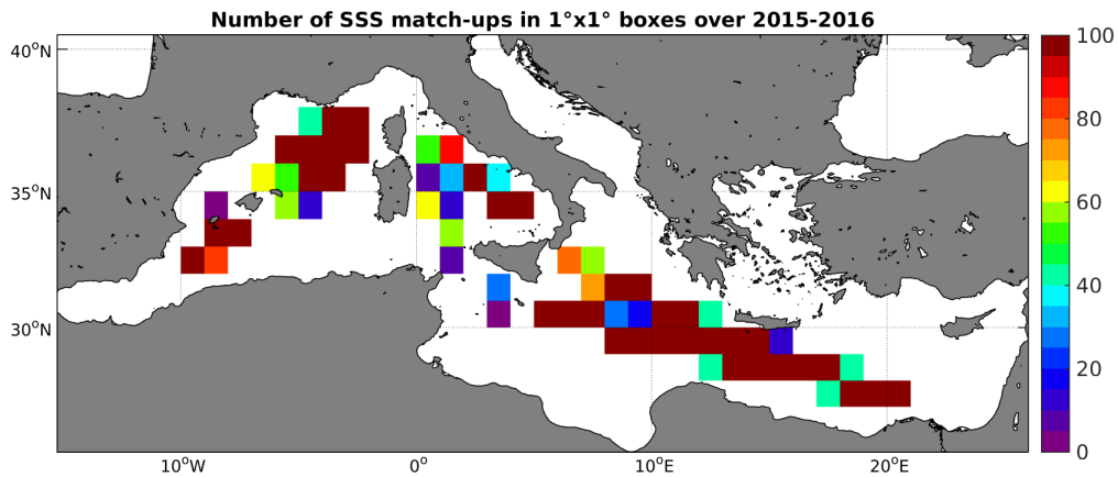
Figure 4: Number of SSS match-ups between TSG-LEGOS-DM SSS and the SMAP-L3-RSS-V2-8DAY-RUNNING-70KM SSS product for the Mediterranean Sea Pi-MEP region over 1^\circ \times 1^\circ boxes and for the full satellite product period.
