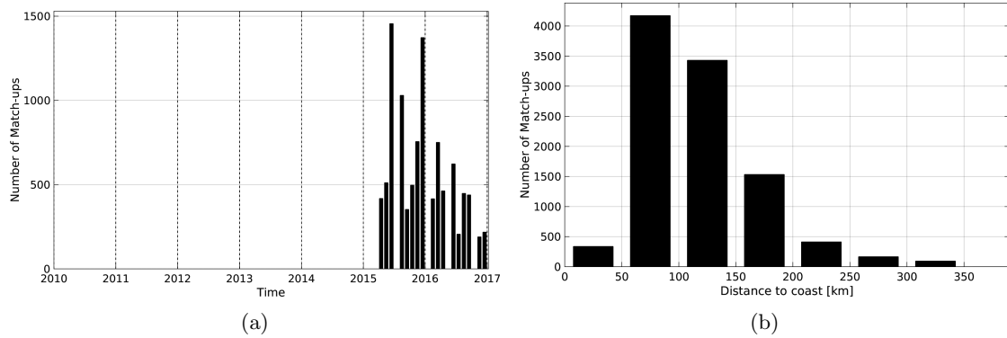
Figure 1: Number of match-ups between TSG-LEGOS-DM and SMAP-L3-RSS-V2-8DAY-RUNNING-70KM SSS as a function of time (a) and as function of the distance to coast (b) over the Mediterranean Sea Pi-MEP region and for the full satellite product period.
