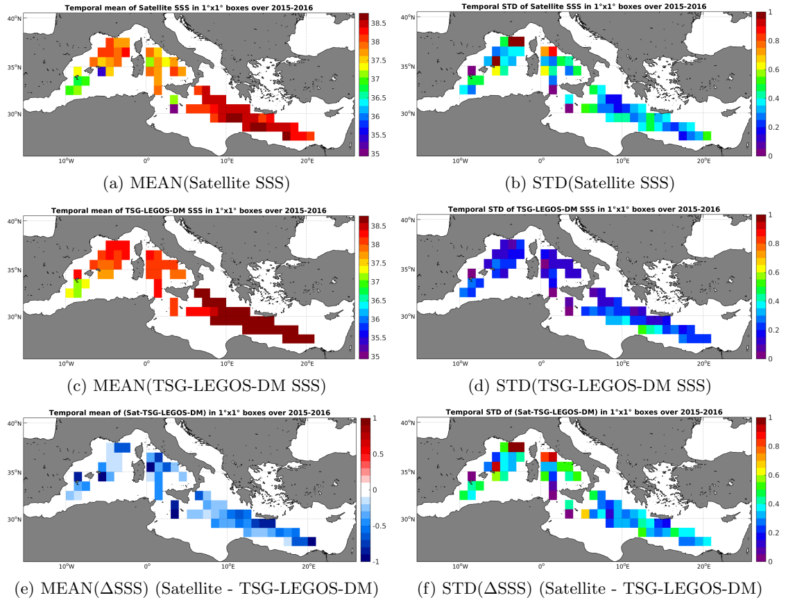
Figure 6: Temporal mean (left) and STD (right) of SSS from SMAP-L3-RSS-V2-8DAY-RUNNING-70KM (top), TSG-LEGOS-DM (middle), and of \Delta SSS (Satellite - TSG-LEGOS-DM). Only match-up pairs are used to generate these maps.
