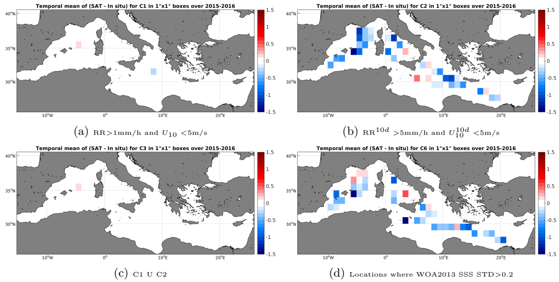
Figure 12: Temporal mean gridded over spatial boxes of size 1^\circ \times 1^\circ of \Delta SSS (SMAP-L3-RSS-V2-8DAY-RUNNING-70KM - TSG-LEGOS-DM) for 4 different subdatasets corresponding to: RR > 1mm/h and U_{10} < 5m/s (a), RR 10d > 5mm/h and U_{10}^{10d} < 5m/s (b), C1 U C2 (c), Locations where WOA2013 SSS STD > 0.2 (d).
