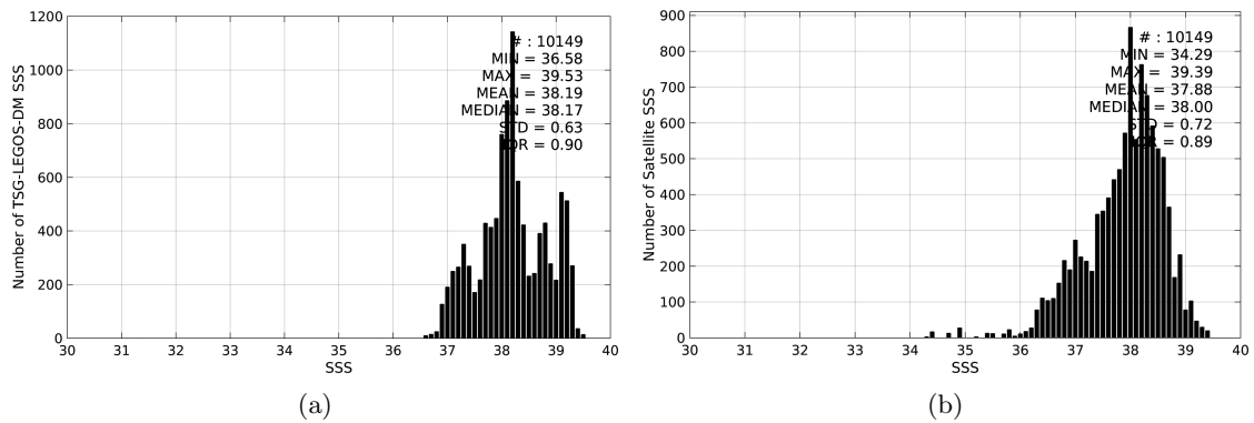
Figure 2: Histograms of SSS from TSG-LEGOS-DM (a) and SMAP-L3-RSS-V2-8DAY-RUNNING-70KM (b) considering all match-up pairs per bins of 0.1 over the Mediterranean Sea Pi-MEP region and for the full satellite product period.
