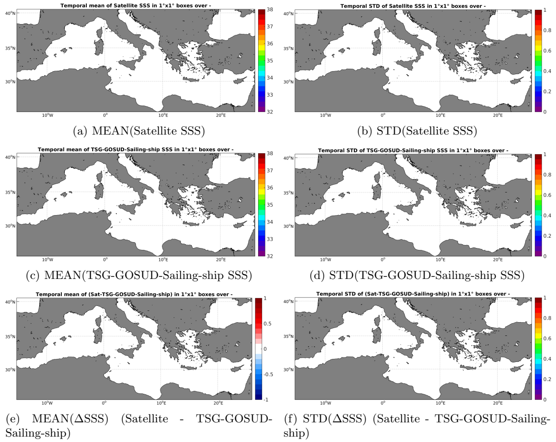
Figure 6: Temporal mean (left) and STD (right) of SSS from SMAP-L3-RSS-V2-8DAY-RUNNING-70KM (top), TSG-GOSUD-Sailing-ship (middle), and of \Delta SSS (Satellite - TSG-GOSUD-Sailing-ship). Only match-up pairs are used to generate these maps.
