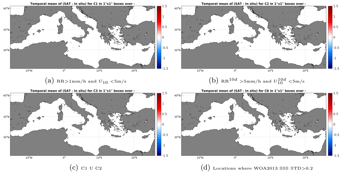
Figure 11: Temporal mean gridded over spatial boxes of size 1^\circ \times 1^\circ of \Delta SSS (SMAP-L3-RSS-V2-8DAY-RUNNING-70KM - Surface drifters) for 4 different subdatasets corresponding to: RR > 1\text{mm/h} and U_{10} < 5\text{m/s} (a), RR^{10d} > 5\text{mm/h} and U_{10}^{10d} < 5\text{m/s} (b), C1 U C2 (c), Locations where WOA2013 SSS STD > 0.2 (d).
