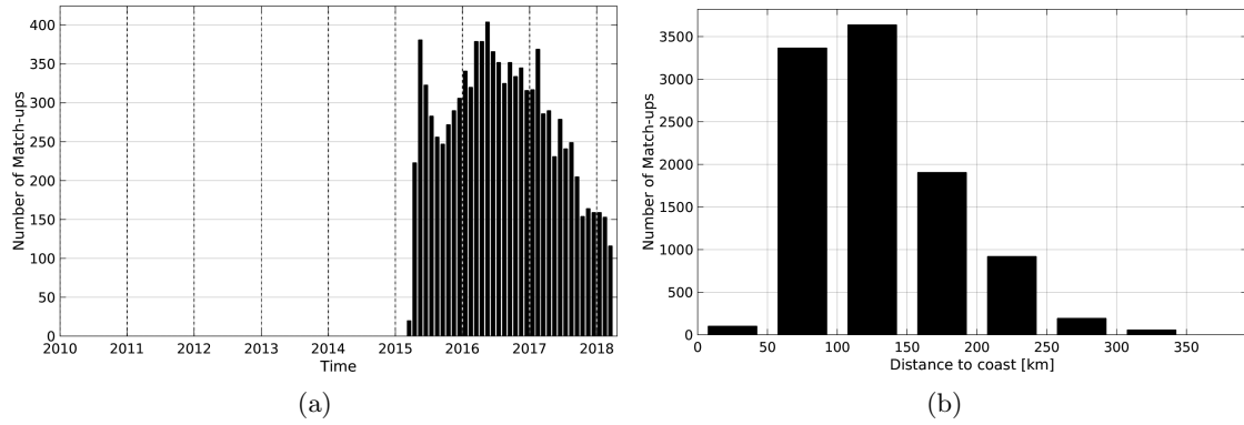
Figure 1: Number of match-ups between Argo and SMAP-L3-RSS-V2-8DAY-RUNNING-70KM SSS as a function of time (a) and as function of the distance to coast (b) over the Mediterranean Sea Pi-MEP region and for the full satellite product period.
