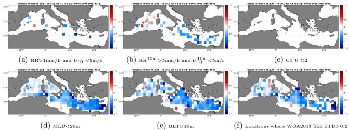
Figure 12: Temporal mean gridded over spatial boxes of size 1^\circ \times 1^\circ of \Delta SSS (SMAP-L3-RSS-V2-8DAY-RUNNING-70KM - Argo) for 6 different subdatasets corresponding to:RR>1mm/h and U_{10} < 5\text{m/s} (a), RR^{10d} > 5\text{mm/h} and U_{10}^{10d} < 5\text{m/s} (b), C1 U C2 (c),MLD<20m (d),BLT>10m (e),Locations where WOA2013 SSS STD>0.2 (f).
