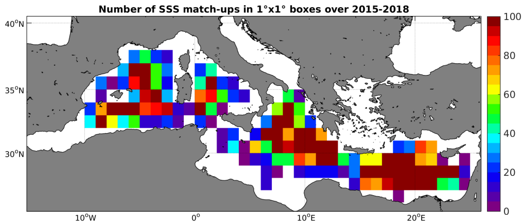
Figure 4: Number of SSS match-ups between Argo SSS and the SMAP-L3-RSS-V2-8DAY-RUNNING-70KM SSS product for the Mediterranean Sea Pi-MEP region over 1^\circ \times 1^\circ boxes and for the full satellite product period.
