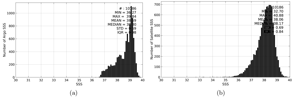
Figure 2: Histograms of SSS from Argo (a) and SMAP-L3-RSS-V2-8DAY-RUNNING-70KM (b) considering all match-up pairs per bins of 0.1 over the Mediterranean Sea Pi-MEP region and for the full satellite product period.
