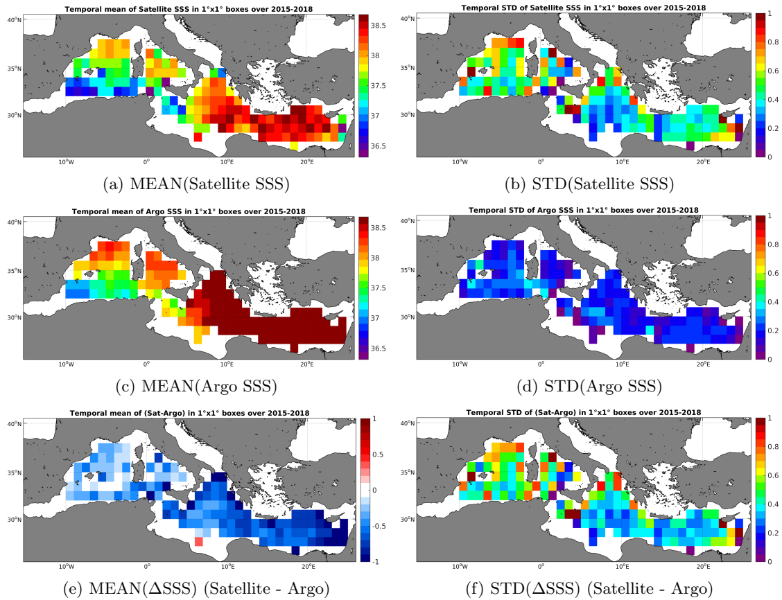
Figure 6: Temporal mean (left) and STD (right) of SSS from SMAP-L3-RSS-V2-8DAY-RUNNING-70KM (top), Argo (middle), and of \Delta SSS (Satellite - Argo). Only match-up pairs are used to generate these maps.
