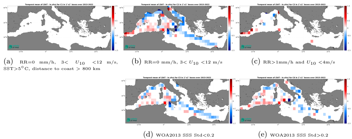
Figure 14: Temporal mean gridded over spatial boxes of size 1^\circ \times 1^\circ of \Delta SSS (SMAP SSS L3 v5.0 - 8-Day running (JPL) - TSG (LEGOS-DM)) for 5 different subdatasets corresponding to:RR=0 mm/h, 3 < U_{10} < 12 m/s, SST >5^\circ\text{C} , distance to coast > 800 km (a), RR=0 mm/h, 3 < U_{10} < 12 m/s (b), RR >1 mm/h and U_{10} < 4 m/s (c), WOA2013 SSS Std <0.2 (d), WOA2013 SSS Std >0.2 (e).
