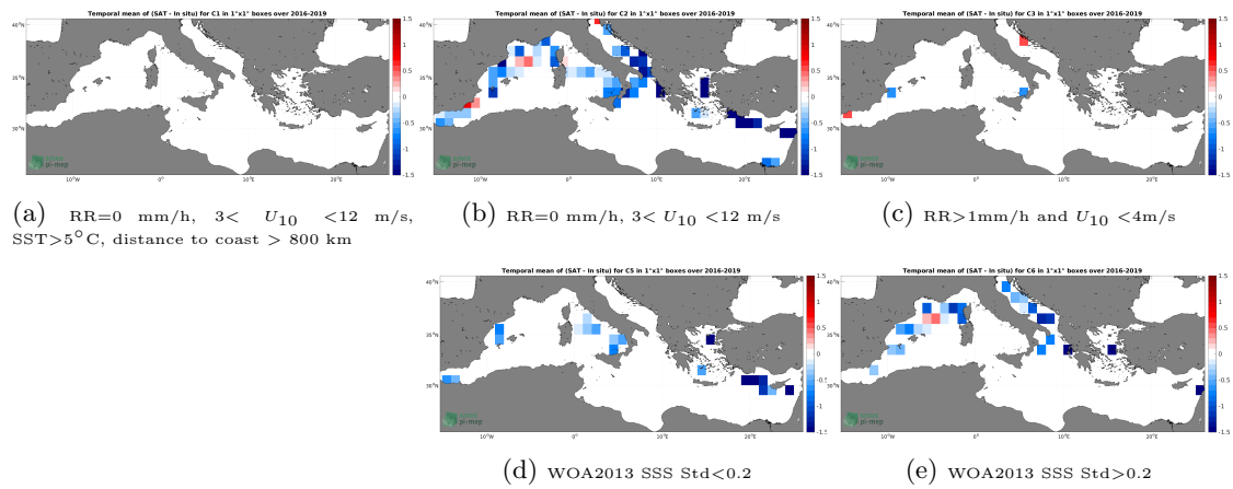
Figure 12: Temporal mean gridded over spatial boxes of size 1^\circ \times 1^\circ of \Delta SSS (SMAP SSS L3 v5.0 - 8-Day running (JPL) - TSG (GOSUD-Sailing-ship)) for 5 different subdatasets corresponding to:RR=0 mm/h, 3 < U_{10} < 12 m/s, SST >5^\circ\text{C} , distance to coast > 800 km (a), RR=0 mm/h, 3 < U_{10} < 12 m/s (b), RR >1 mm/h and U_{10} < 4 m/s (c), WOA2013 SSS Std <0.2 (d), WOA2013 SSS Std >0.2 (e).
