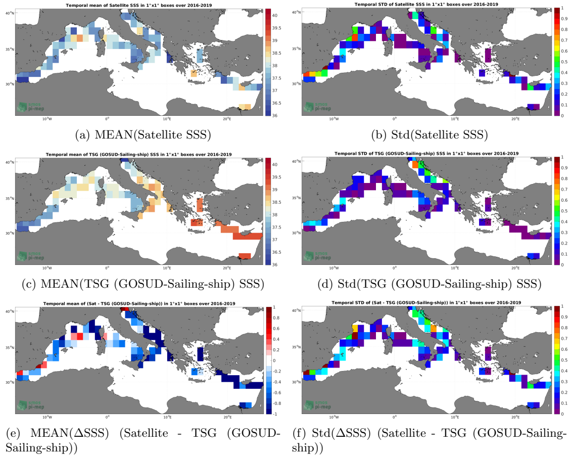
Figure 6: Temporal mean (left) and Std (right) of SSS from SMAP SSS L3 v5.0 - 8-Day running (JPL) (top), TSG (GOSUD-Sailing-ship) (middle), and of \Delta SSS (Satellite - TSG (GOSUD-Sailing-ship)). Only match-up pairs are used to generate these maps.
