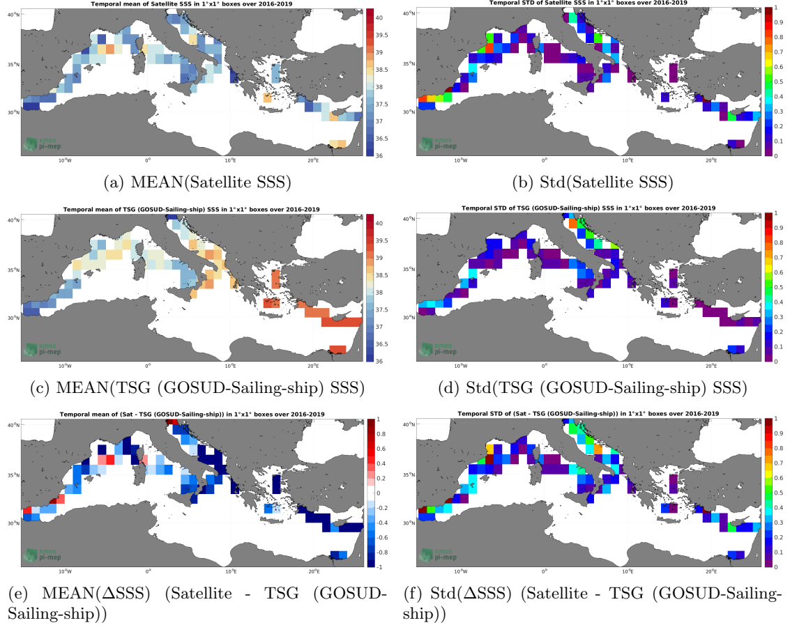
Figure 6: Temporal mean (left) and Std (right) of SSS from SMAP SSS L3 v5.0 - 8-Day running (JPL) (top), TSG (GOSUD-Sailing-ship) (middle), and of \Delta\text{SSS} (Satellite - TSG (GOSUD-Sailing-ship)). Only match-up pairs are used to generate these maps.
