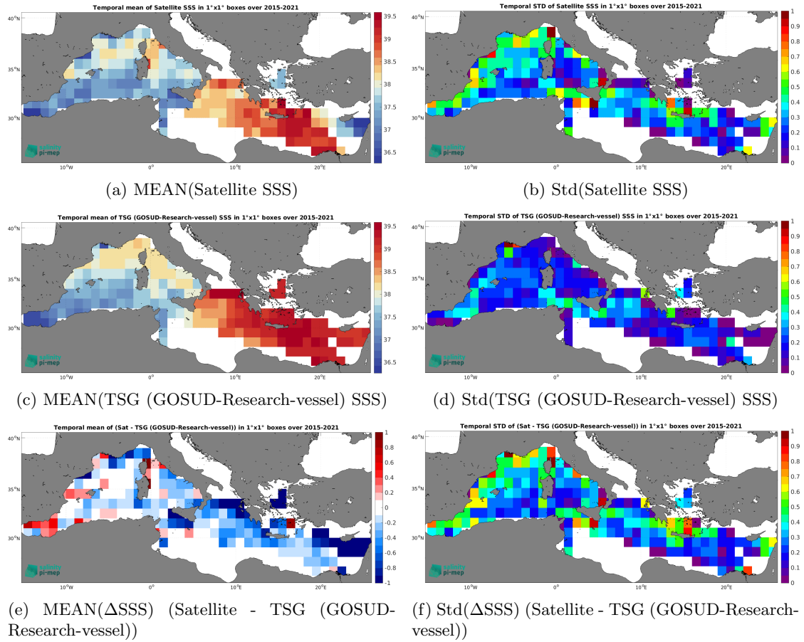
Figure 6: Temporal mean (left) and Std (right) of SSS from SMAP SSS L3 v5.0 - 8-Day running (JPL) (top), TSG (GOSUD-Research-vessel) (middle), and of \Delta SSS (Satellite - TSG (GOSUD-Research-vessel)). Only match-up pairs are used to generate these maps.
