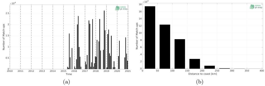
Figure 1: Number of match-ups between TSG (GOSUD-Research-vessel) and SMAP SSS L3 v5.0 - 8-Day running (JPL) SSS as a function of time (a) and as function of the distance to coast (b) over the Mediterranean Sea Pi-MEP region and for the full satellite product period.
