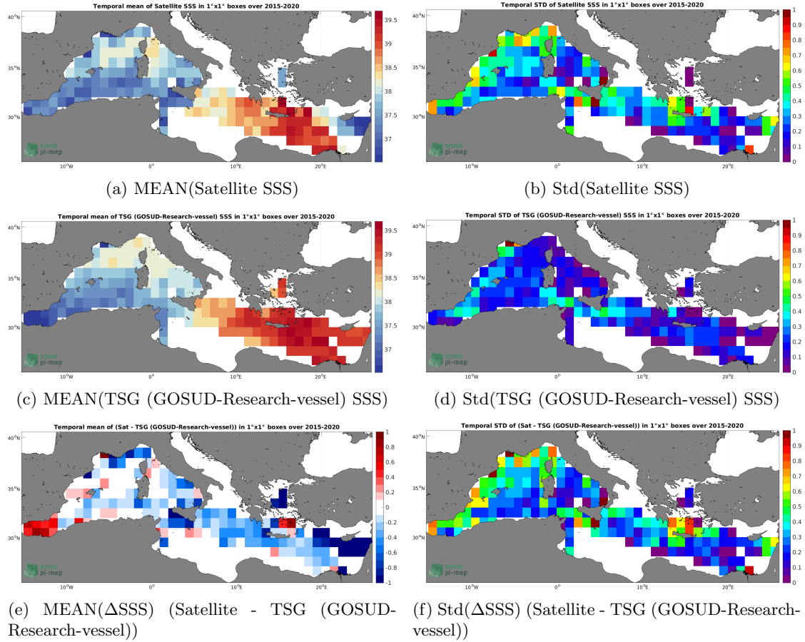
Figure 6: Temporal mean (left) and Std (right) of SSS from SMAP SSS L3 v5.0 - 8-Day running (JPL) (top), TSG (GOSUD-Research-vessel) (middle), and of \Delta SSS (Satellite - TSG (GOSUD-Research-vessel)). Only match-up pairs are used to generate these maps.
