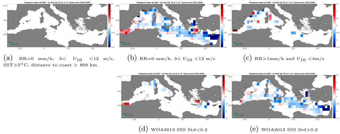
Figure 12: Temporal mean gridded over spatial boxes of size 1^{\circ}\times 1^{\circ} of \Delta SSS (SMAP SSS L3 v5.0 - 8-Day running (JPL) - TSG (GOSUD-Research-vessel)) for 5 different subdatasets corresponding to:RR=0 mm/h, 3 < U_{10} < 12 m/s, SST >5^{\circ}\text{C} , distance to coast > 800 km (a), RR=0 mm/h, 3 < U_{10} < 12 m/s (b), RR >1 mm/h and U_{10} < 4 m/s (c), WOA2013 SSS Std <0.2 (d), WOA2013 SSS Std >0.2 (e).
