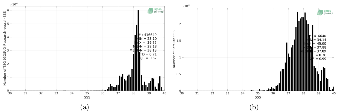
Figure 2: Histograms of SSS from TSG (GOSUD-Research-vessel) (a) and SMAP SSS L3 v5.0 - 8-Day running (JPL) (b) considering all match-up pairs per bins of 0.1 over the Mediterranean Sea Pi-MEP region and for the full satellite product period.
