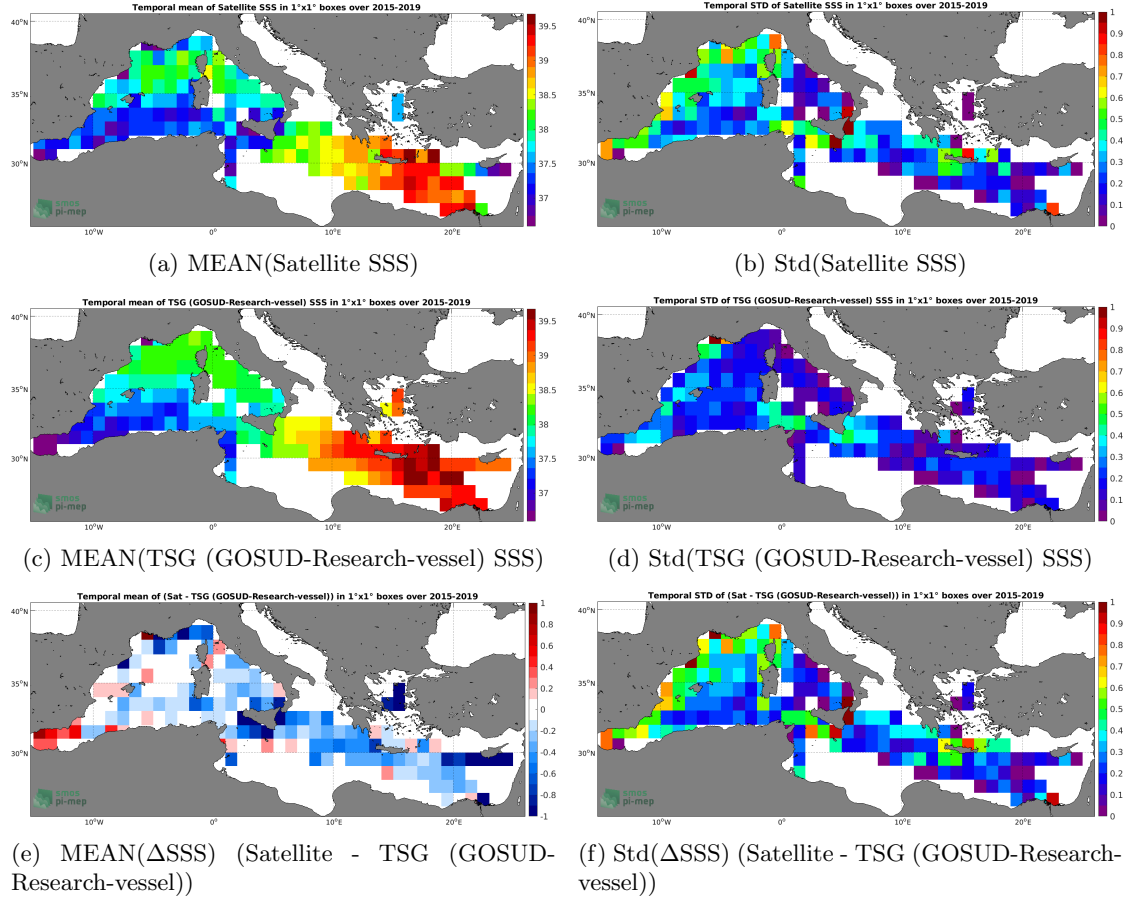
Figure 6: Temporal mean (left) and Std (right) of SSS from SMAP SSS L3 v5.0 - 8-Day running (JPL) (top), TSG (GOSUD-Research-vessel) (middle), and of \Delta\text{SSS} (Satellite - TSG (GOSUD-Research-vessel)). Only match-up pairs are used to generate these maps.
