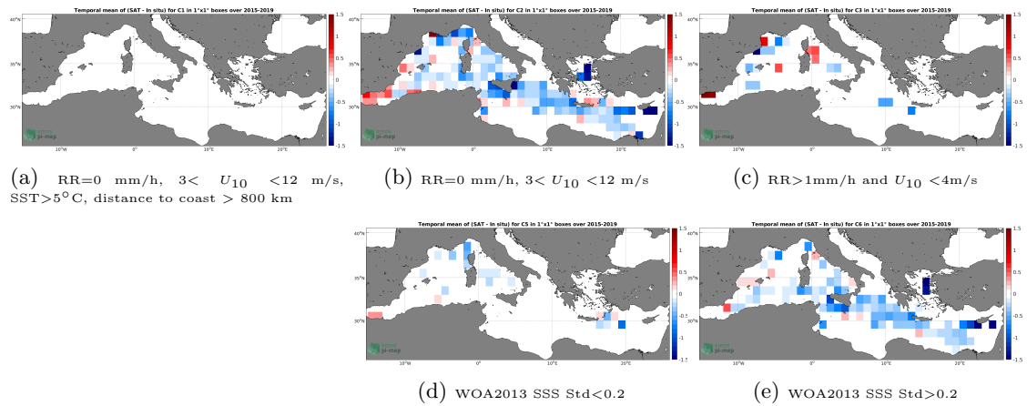
Figure 12: Temporal mean gridded over spatial boxes of size 1^\circ \times 1^\circ of \Delta SSS (SMAP SSS L3 v5.0 - 8-Day running (JPL) - TSG (GOSUD-Research-vessel)) for 5 different subdatasets corresponding to:RR=0 mm/h, 3 < U_{10} < 12 m/s, SST >5^\circ\text{C} , distance to coast > 800 km (a), RR=0 mm/h, 3 < U_{10} < 12 m/s (b), RR >1 mm/h and U_{10} < 4 m/s (c), WOA2013 SSS Std <0.2 (d), WOA2013 SSS Std >0.2 (e).
