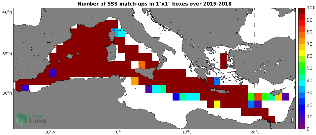
Figure 4: Number of SSS match-ups between TSG (GOSUD-Research-vessel) SSS and the SMAP SSS L3 v5.0 - 8-Day running (JPL) SSS product for the Mediterranean Sea Pi-MEP region over 1°x1° boxes and for the full satellite product period.
