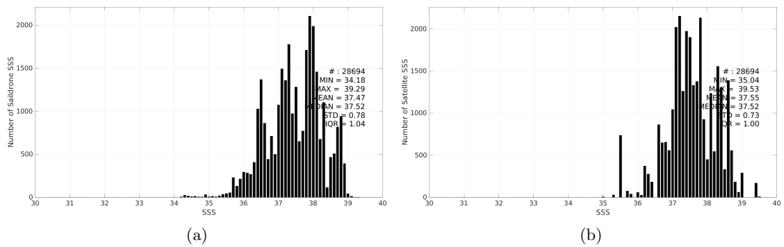
Figure 3: Histograms of SSS from Saildrone (a) and SMAP SSS L3 v5.0 - 8-Day running (JPL) (b) considering all match-up pairs per bins of 0.1 over the Mediterranean Sea Pi-MEP region and for the full satellite product period.
