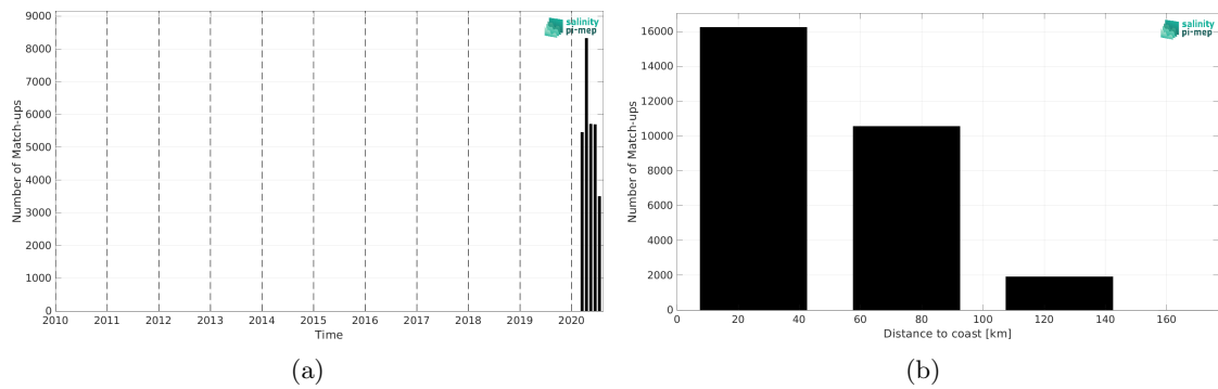
Figure 2: Number of match-ups between Saildrone and SMAP SSS L3 v5.0 - 8-Day running (JPL) SSS as a function of time (a) and as function of the distance to coast (b) over the Mediterranean Sea Pi-MEP region and for the full satellite product period.
