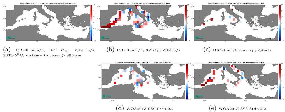
Figure 14: Temporal mean gridded over spatial boxes of size 1^\circ \times 1^\circ of \Delta\text{SSS} (SMAP SSS L3 v5.0 - 8-Day running (JPL) - Saildrone) for 5 different subdatasets corresponding to:RR=0 mm/h, 3 < U_{10} < 12 m/s, SST>5°C, distance to coast > 800 km (a), RR=0 mm/h, 3 < U_{10} < 12 m/s (b), RR>1mm/h and U_{10} < 4 m/s (c), WOA2013 SSS Std<0.2 (d), WOA2013 SSS Std>0.2 (e).
