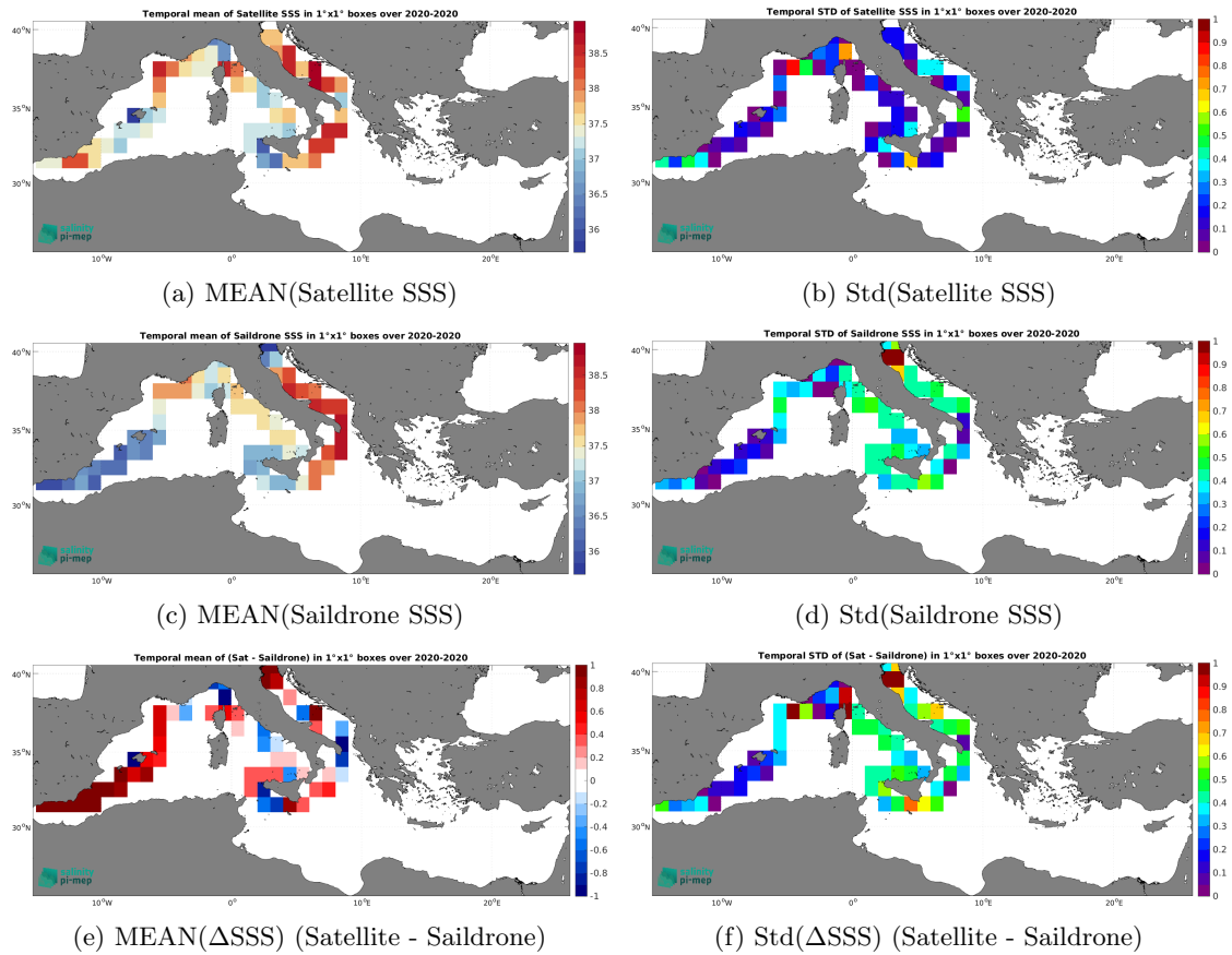
Figure 7: Temporal mean (left) and Std (right) of SSS from SMAP SSS L3 v5.0 - 8-Day running (JPL) (top), Saildrone (middle), and of \Delta SSS (Satellite - Saildrone). Only match-up pairs are used to generate these maps.
