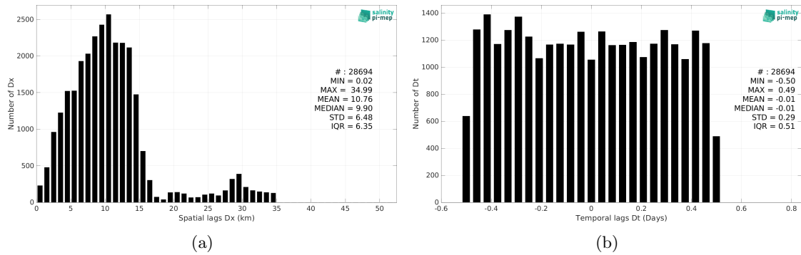
Figure 6: Histograms of the spatial (a) and temporal (b) lags between the location/time of the Sairdrona measurement and the date of the corresponding SMAP SSS L3 v5.0 - 8-Day running (JPL) SSS pixel.
