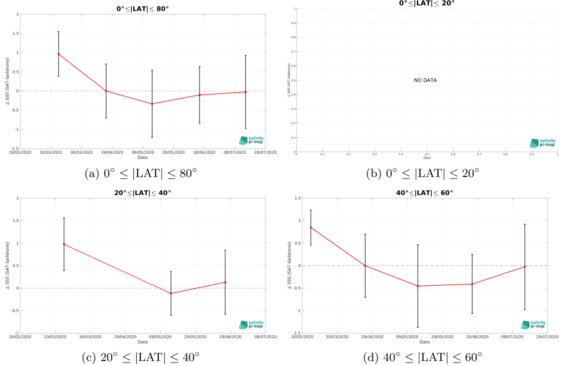
Figure 11: Monthly median (red curves) of \Delta\text{SSS} (Satellite - Sailability) and \pm 1 Std (black vertical thick bars) as function of time for all the collected Pi-MEP match-up pairs estimated over the Mediterranean Sea Pi-MEP region and for the full satellite product period are shown for different latitude bands: (a) 80^{\circ}\text{S}-80^{\circ}\text{N} , (b) 20^{\circ}\text{S}-20^{\circ}\text{N} , (c) 40^{\circ}\text{S}-20^{\circ}\text{S} and 20^{\circ}\text{N}-40^{\circ}\text{N} and (d) 60^{\circ}\text{S}-40^{\circ}\text{S} and 40^{\circ}\text{N}-60^{\circ}\text{N} .
