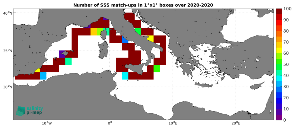
Figure 5: Number of SSS match-ups between Saildrone SSS and the SMAP SSS L3 v5.0 - 8-Day running (JPL) SSS product for the Mediterranean Sea Pi-MEP region over 1^\circ \times 1^\circ boxes and for the full satellite product period.
