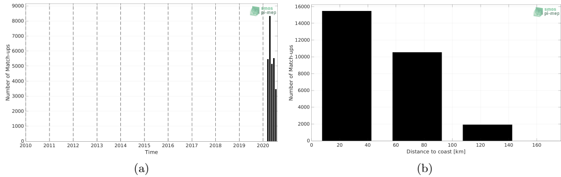
Figure 1: Number of match-ups between Saildrone and SMAP SSS L3 v5.0 - 8-Day running (JPL) SSS as a function of time (a) and as function of the distance to coast (b) over the Mediterranean Sea Pi-MEP region and for the full satellite product period.
