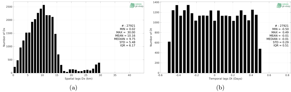
Figure 5: Histograms of the spatial (a) and temporal (b) lags between the location/time of the Smaildrone measurement and the date of the corresponding SMAP SSS L3 v5.0 - 8-Day running (JPL) SSS pixel.
