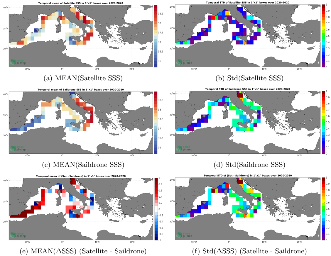
Figure 6: Temporal mean (left) and Std (right) of SSS from SMAP SSS L3 v5.0 - 8-Day running (JPL) (top), Saildrone (middle), and of \Delta SSS (Satellite - Saildrone). Only match-up pairs are used to generate these maps.
