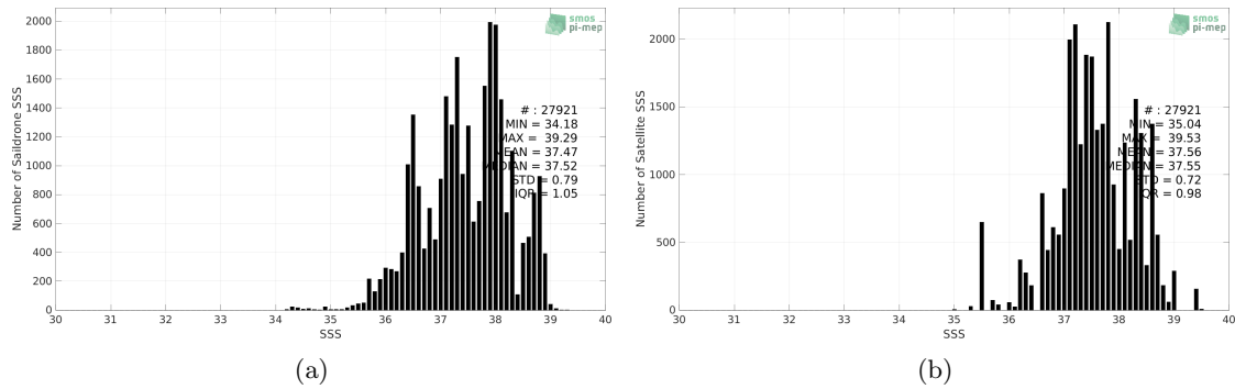
Figure 2: Histograms of SSS from Saildrone (a) and SMAP SSS L3 v5.0 - 8-Day running (JPL) (b) considering all match-up pairs per bins of 0.1 over the Mediterranean Sea Pi-MEP region and for the full satellite product period.
