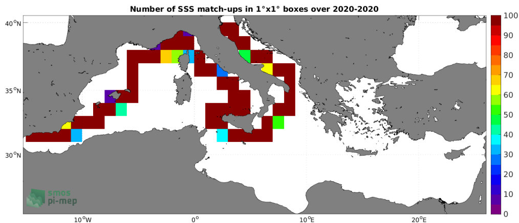
Figure 4: Number of SSS match-ups between Saildrone SSS and the SMAP SSS L3 v5.0 - 8-Day running (JPL) SSS product for the Mediterranean Sea Pi-MEP region over 1^\circ \times 1^\circ boxes and for the full satellite product period.
