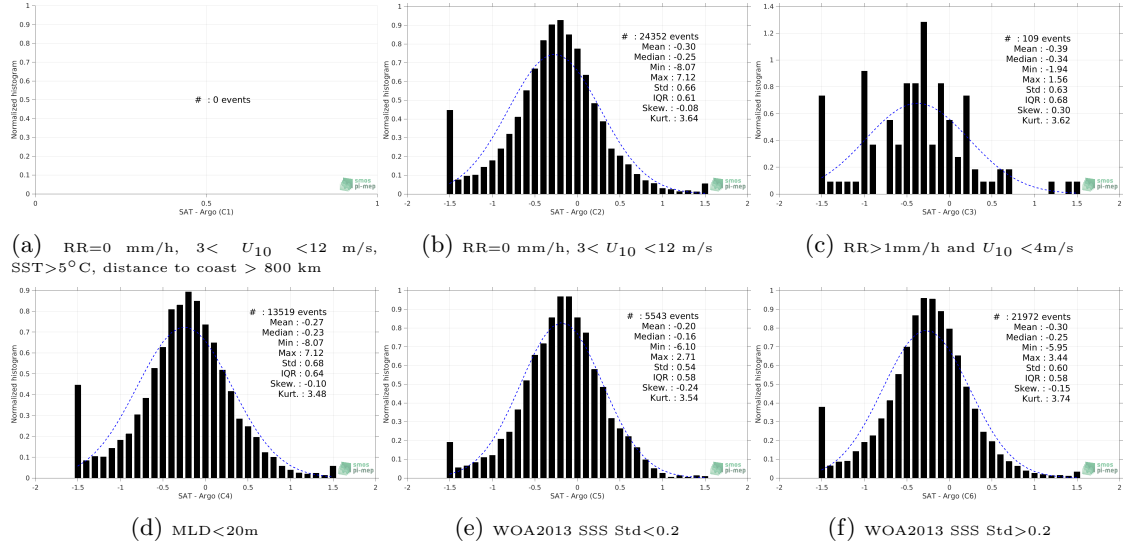
Figure 13: Normalized histogram of \Delta SSS (SMAP SSS L3 v5.0 - 8-Day running (JPL) - Argo) for 6 different subdatasets corresponding to: RR=0 mm/h, 3 < U_{10} < 12 m/s, SST > 5^\circ C , distance to coast > 800 km (a), RR=0 mm/h, 3 < U_{10} < 12 m/s (b), RR > 1 mm/h and U_{10} < 4 m/s (c), MLD < 20 m (d), WOA2013 SSS Std < 0.2 (e), WOA2013 SSS Std > 0.2 (f).
