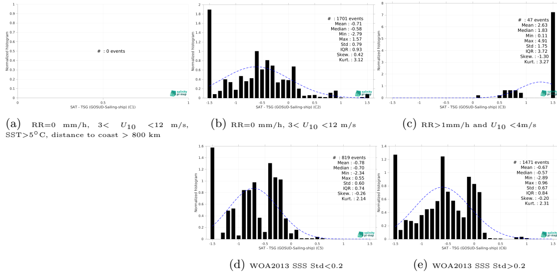
Figure 15: Normalized histogram of \Delta\text{SSS} (SMAP SSS L3 v5.0 - Monthly (JPL) - TSG (GOSUD-Sailing-ship)) for 5 different subdatasets corresponding to: RR=0 mm/h, 3 < U_{10} < 12 m/s, SST > 5^{\circ}\text{C} , distance to coast > 800 km (a), RR=0 mm/h, 3 < U_{10} < 12 m/s (b), RR > 1\text{mm/h} and U_{10} < 4\text{m/s} (c), WOA2013 SSS Std < 0.2 (d), WOA2013 SSS Std > 0.2 (e).
