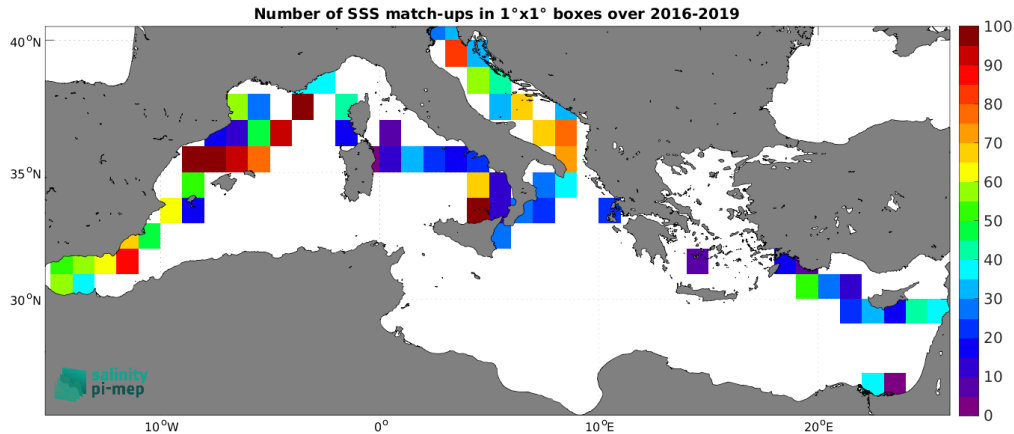
Figure 5: Number of SSS match-ups between TSG (GOSUD-Sailing-ship) SSS and the SMAP SSS L3 v5.0 - Monthly (JPL) SSS product for the Mediterranean Sea Pi-MEP region over 1^\circ \times 1^\circ boxes and for the full satellite product period.
