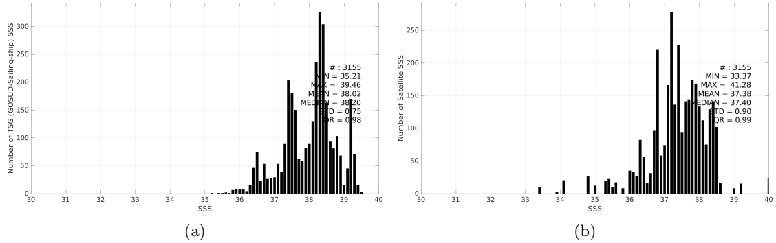
Figure 3: Histograms of SSS from TSG (GOSUD-Sailing-ship) (a) and SMAP SSS L3 v5.0 - Monthly (JPL) (b) considering all match-up pairs per bins of 0.1 over the Mediterranean Sea Pi-MEP region and for the full satellite product period.
