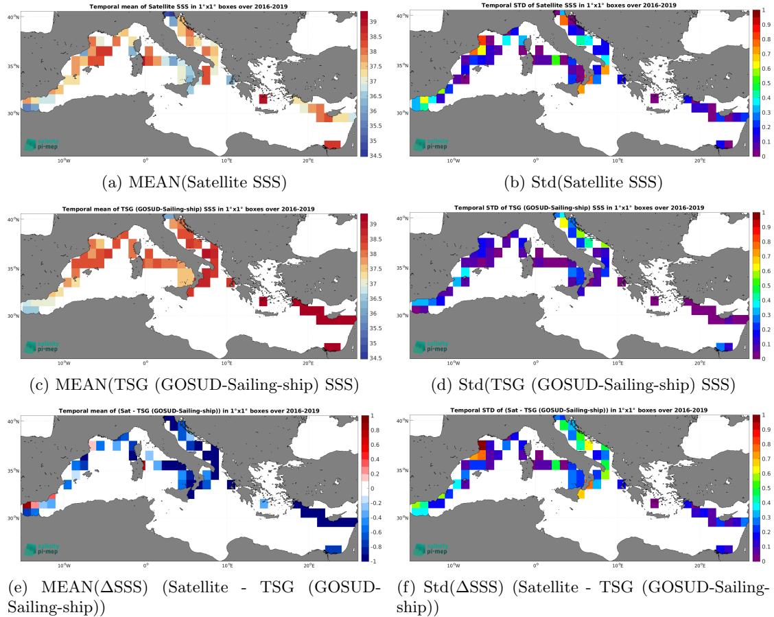
Figure 7: Temporal mean (left) and Std (right) of SSS from SMAP SSS L3 v5.0 - Monthly (JPL) (top), TSG (GOSUD-Sailing-ship) (middle), and of \Delta\text{SSS} (Satellite - TSG (GOSUD-Sailing-ship)). Only match-up pairs are used to generate these maps.
