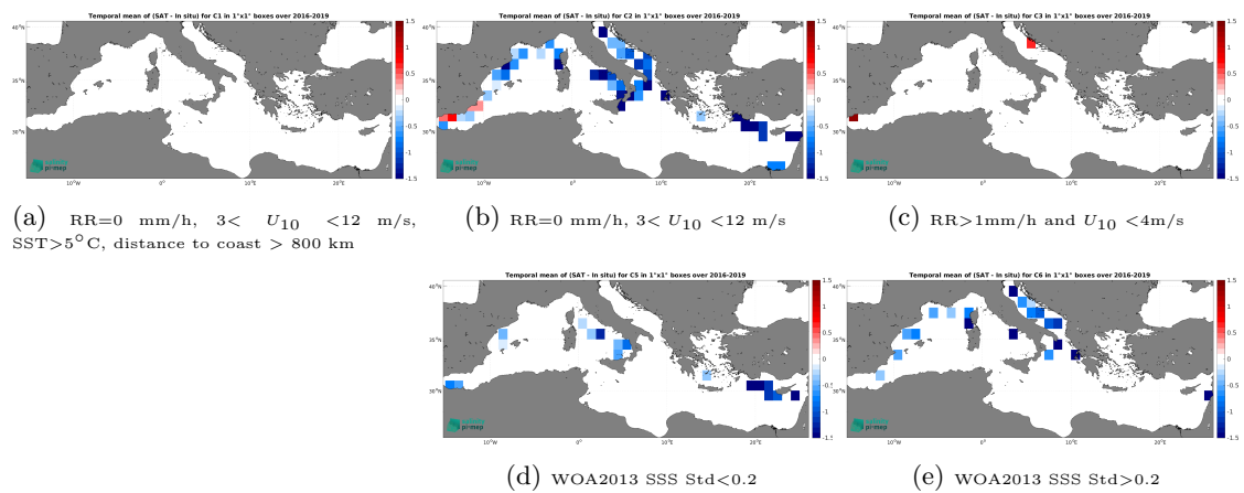
Figure 14: Temporal mean gridded over spatial boxes of size 1^\circ \times 1^\circ of \Delta\text{SSS} (SMAP SSS L3 v5.0 - Monthly (JPL) - TSG (GOSUD-Sailing-ship)) for 5 different subdatasets corresponding to:RR=0 mm/h, 3 < U_{10} < 12 m/s, SST>5°C, distance to coast > 800 km (a), RR=0 mm/h, 3 < U_{10} < 12 m/s (b), RR>1mm/h and U_{10} < 4 m/s (c), WOA2013 SSS Std<0.2 (d), WOA2013 SSS Std>0.2 (e).
