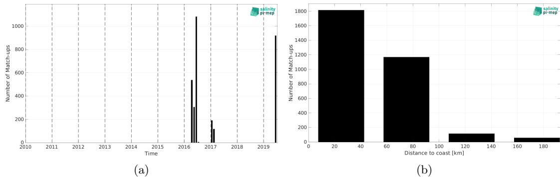
Figure 2: Number of match-ups between TSG (GOSUD-Sailing-ship) and SMAP SSS L3 v5.0 - Monthly (JPL) SSS as a function of time (a) and as function of the distance to coast (b) over the Mediterranean Sea Pi-MEP region and for the full satellite product period.
